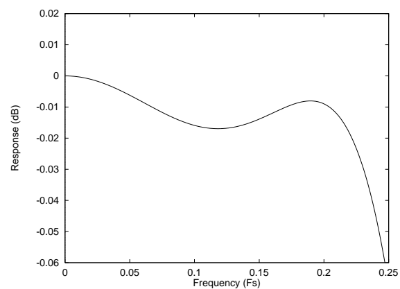
Figure 28 ADC Digital Filter Ripple –Type 3
