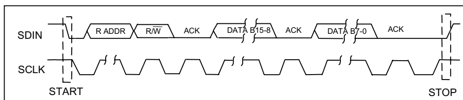
Figure 19 2-Wire Serial Interface
