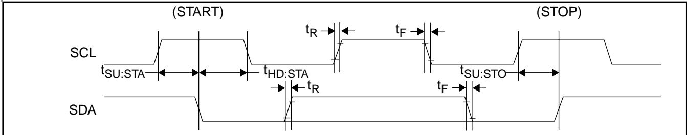
FIGURE 5. Input Timing
