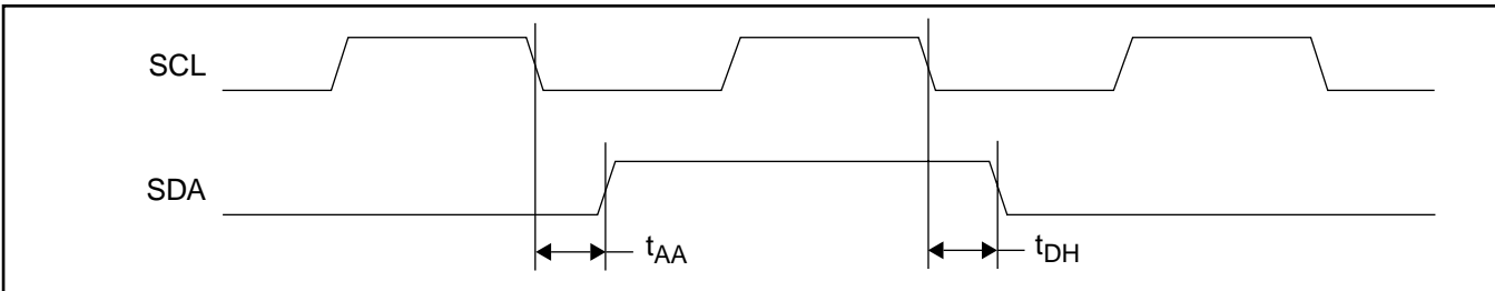
FIGURE 6. Output Timing
