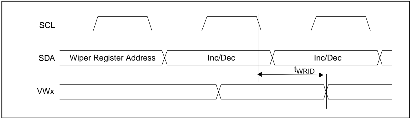
FIGURE 8. EEPOT Timing (for Increment/Decrement Instruction)
