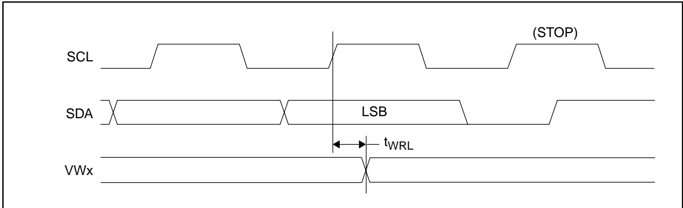
FIGURE 7. EEPOT Timing (for All Load Instructions)
