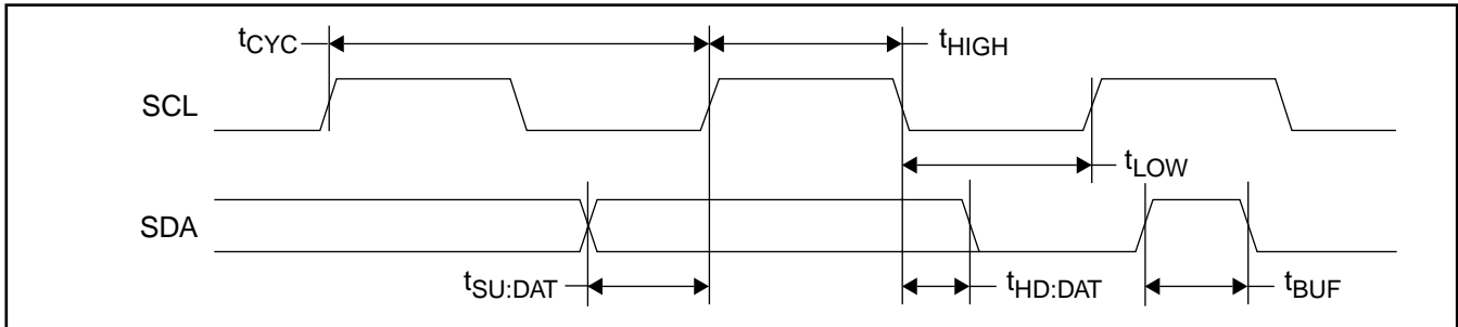
FIGURE 5. Input Timing
