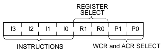
Figure 2. Instruction Byte Format
