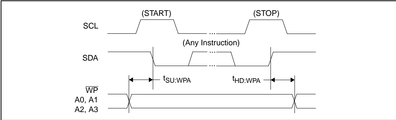
FIGURE 9. Write Protect and Device Address Pins Timing
