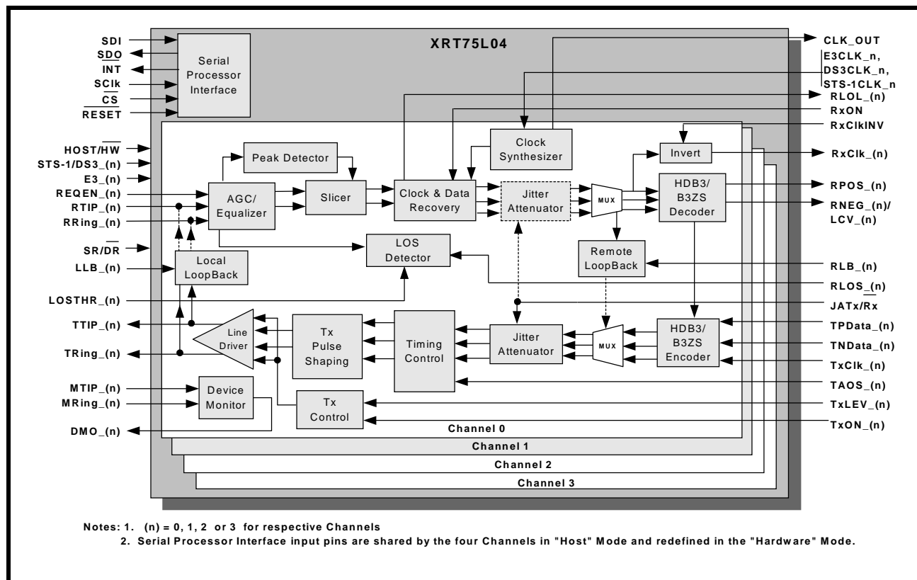
FIGURE 1. BLOCK DIAGRAM OF THE XRT75L04
