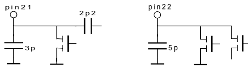
pin21 and 22: clock oscillator
