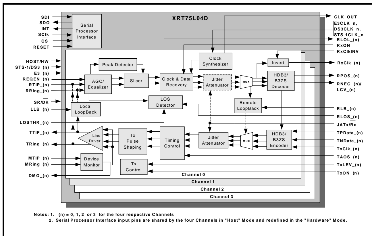
FIGURE 1. BLOCK DIAGRAM OF THE XRT75L04D
