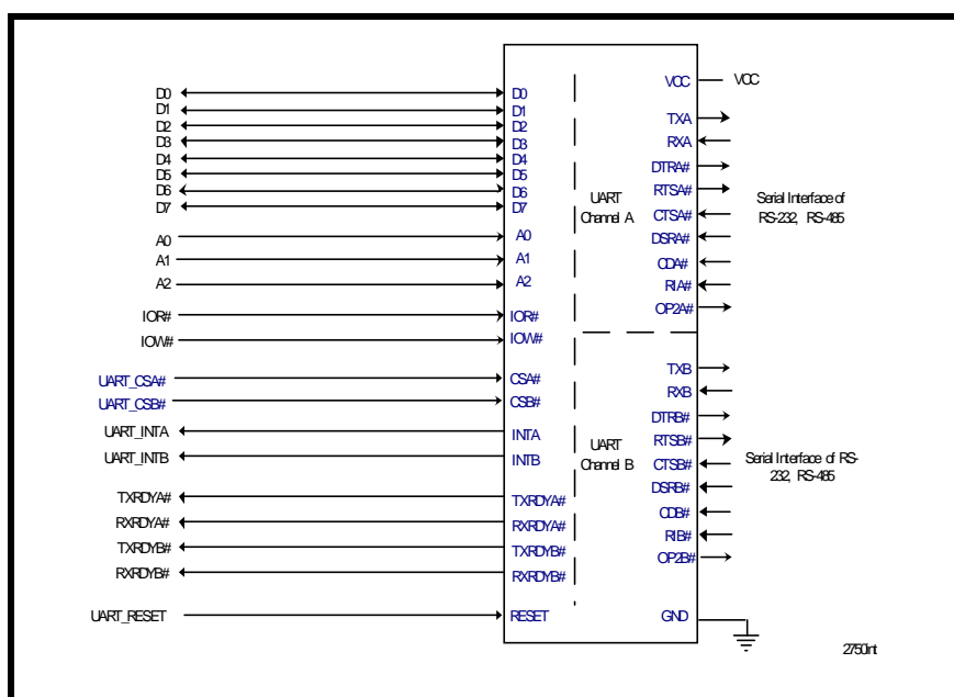
FIGURE 3. XR16L2750 DATA BUS INTERCONNECTIONS
