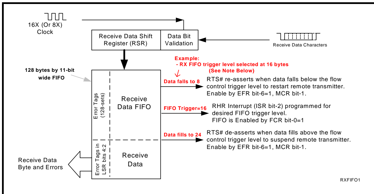
FIGURE 13. RECEIVER OPERATION IN FIFO AND AUTO RTS FLOW CONTROL MODE
