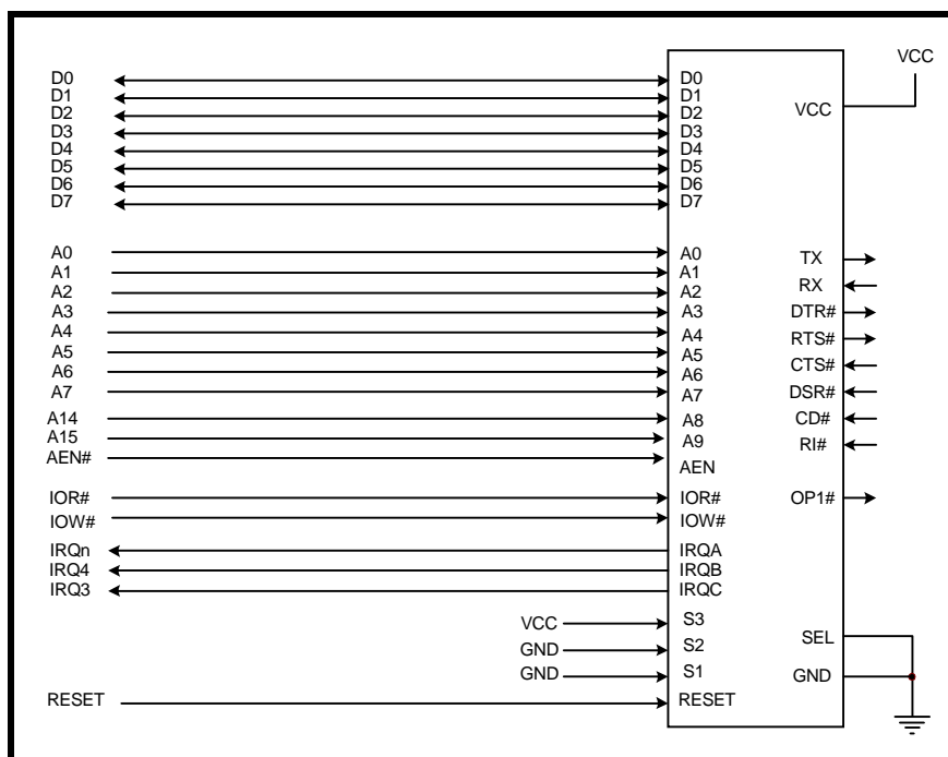
FIGURE 5. XR16C850 PC MODE INTERCONNECTIONS
