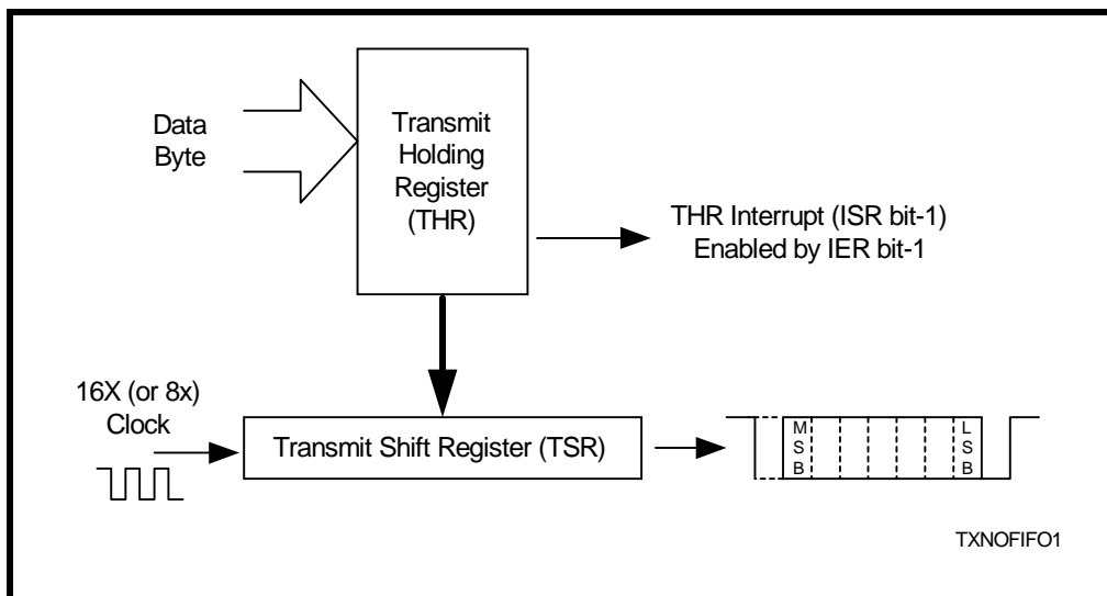
FIGURE 10. TRANSMITTER OPERATION IN NON-FIFO MODE
