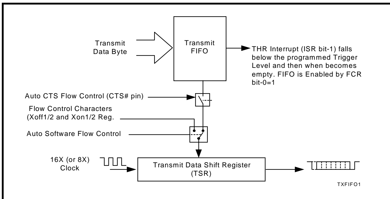
FIGURE 11. TRANSMITTER OPERATION IN FIFO AND FLOW CONTROL MODE
