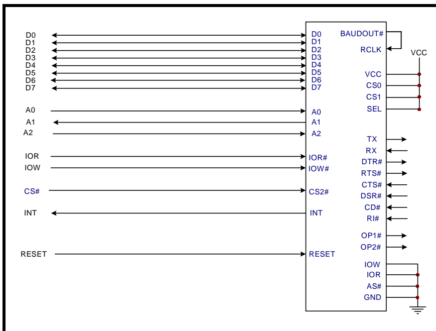
FIGURE 4. XR16C850 INTEL BUS INTERCONNECTIONS
