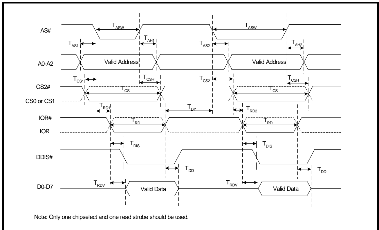
FIGURE 22. DATA BUS READ TIMING IN INTEL BUS MODE USING AS#
