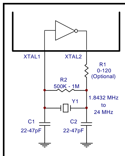
FIGURE 8. TYPICAL OSCILLATOR CONNECTIONS
