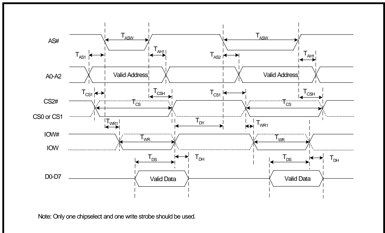
FIGURE 23. DATA BUS WRITE TIMING IN INTEL BUS MODE USING AS#
