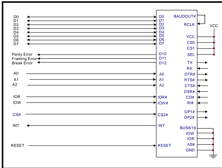
FIGURE 7. XR16C850 16-BIT BUS INTERFACE
