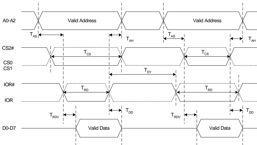
FIGURE 20. DATA BUS READ TIMING IN INTEL BUS MODE WITH AS# TIED TO GND
