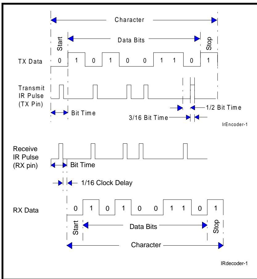
FIGURE 16. INFRARED TRANSMIT DATA ENCODING AND RECEIVE DATA DECODING
