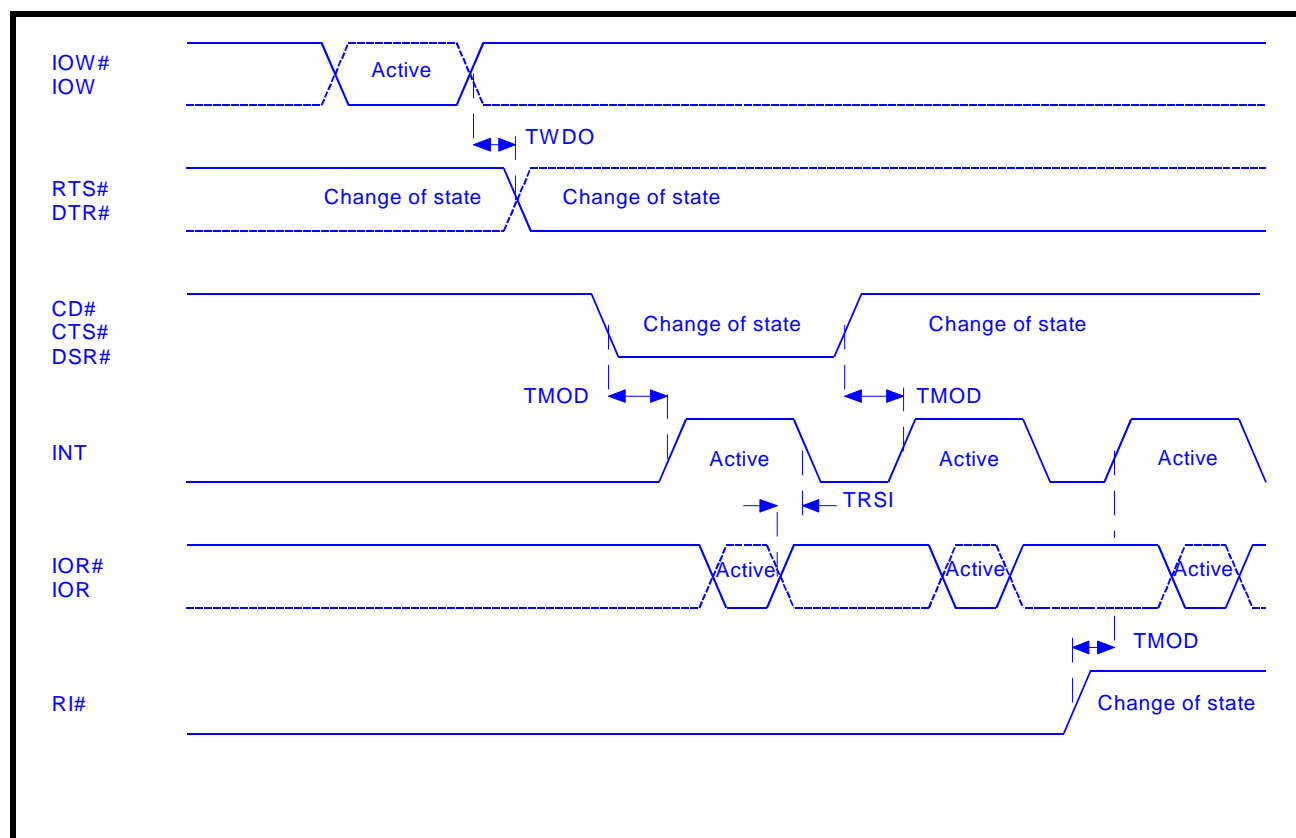
FIGURE 19. MODEM INPUT/OUTPUT TIMING
