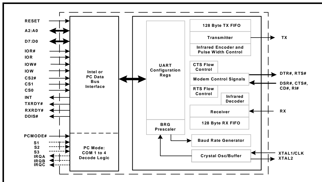
FIGURE 1. BLOCK DIAGRAM
