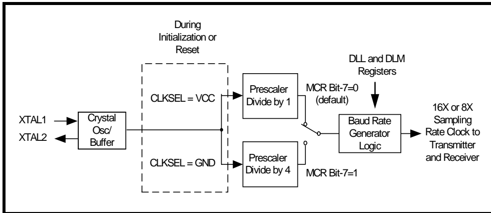
FIGURE 9. BAUD RATE GENERATOR
