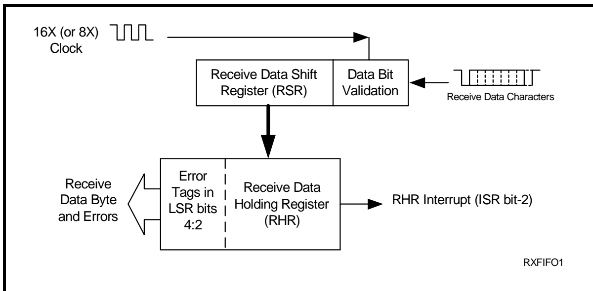
FIGURE 12. RECEIVER OPERATION IN NON-FIFO MODE
