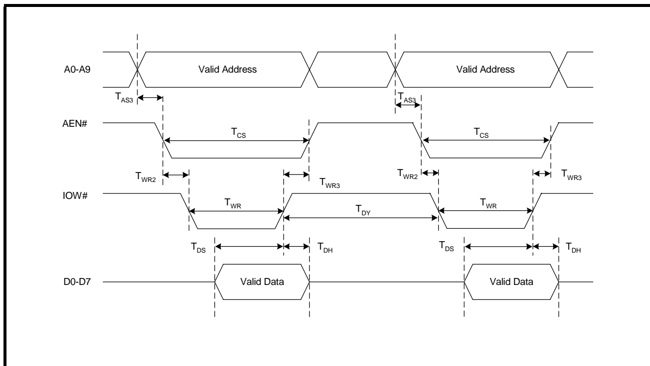
FIGURE 25. DATA BUS WRITE TIMING IN PC MODE
