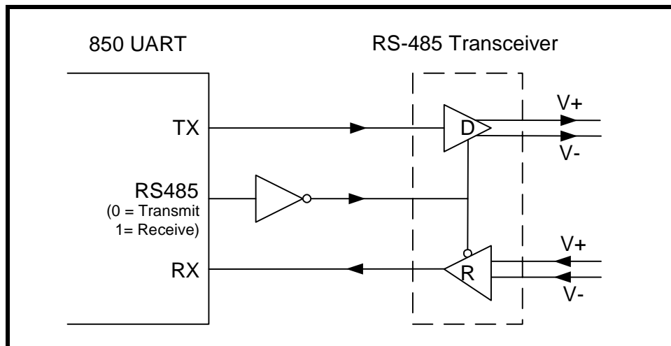
FIGURE 15. AUTO RS-485 HALF-DUPLEX CONTROL
