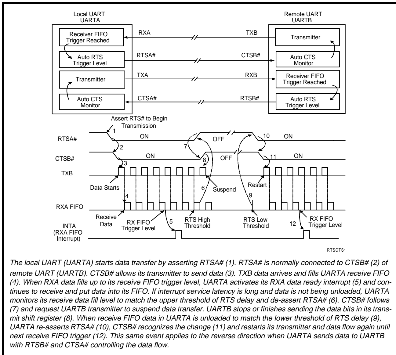
FIGURE 14. AUTO RTS AND CTS FLOW CONTROL OPERATION
