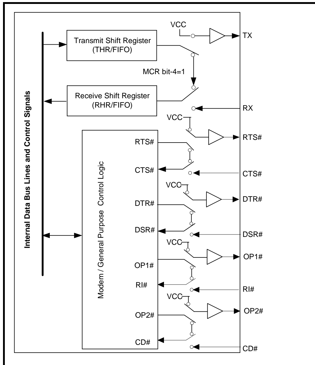
FIGURE 17. INTERNAL LOOPBACK
