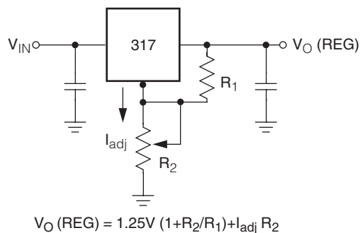
Voltage Regulator
