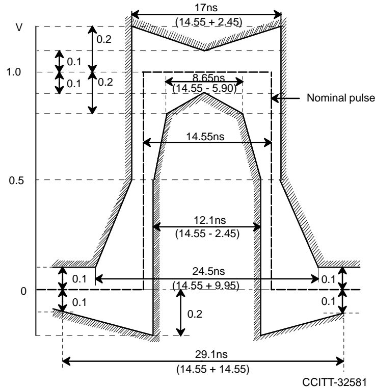
Figure 4. Pulse Mask at the 34.368 Mbit/s Interface
