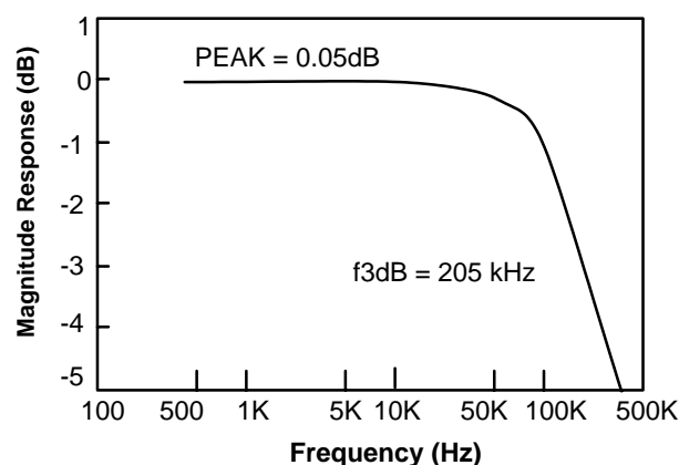
Figure 5. Typical PLL Jitter Transfer Characteristics
