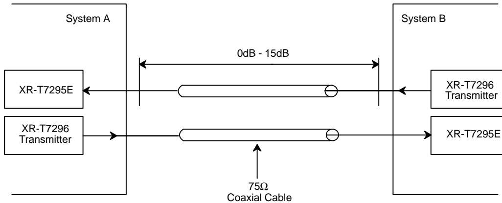
Figure 2. Application Diagram
