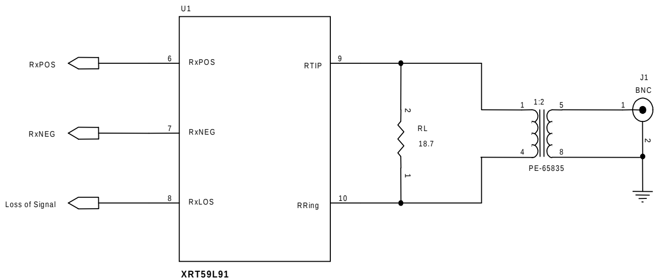
Figure 7. Recommended Schematic for Interfacing the Receive Section of the XRT59L91 Device to the Line for 75W Applications (Transformer-Coupling)
