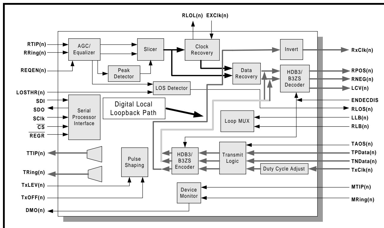
FIGURE 28. ILLUSTRATION OF THE "DIGITAL LOCAL LOOP-BACK" PATH IN A TYPICAL CHANNEL(N) (OF THE XRT7302)
