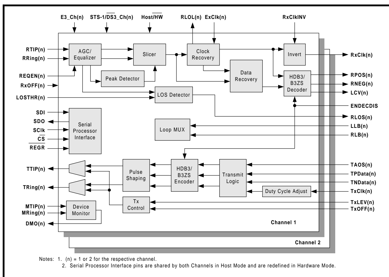
FIGURE 6. FUNCTIONAL BLOCK DIAGRAM OF THE XRT7302
