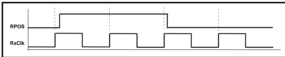
FIGURE 26. ILLUSTRATION OF THE BEHAVIOR OF THE RPOS AND RxCCLK OUTPUT SIGNALS, WHILE THE XRT7302 IS TRANSMITTING "SINGLE-RAIL" DATA TO THE RECEIVING TERMINAL EQUIPMENT
