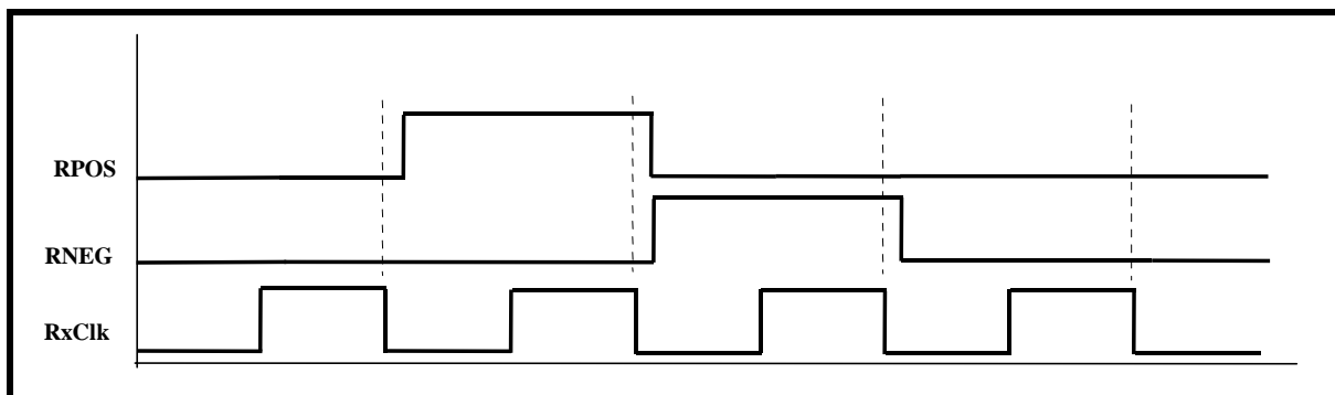
FIGURE 24. ILLUSTRATION OF THE BEHAVIOR OF THE RPOS, RNEG, AND RXCLK(N) SIGNALS, WHEN RXCLK(N) IS INVERTED
