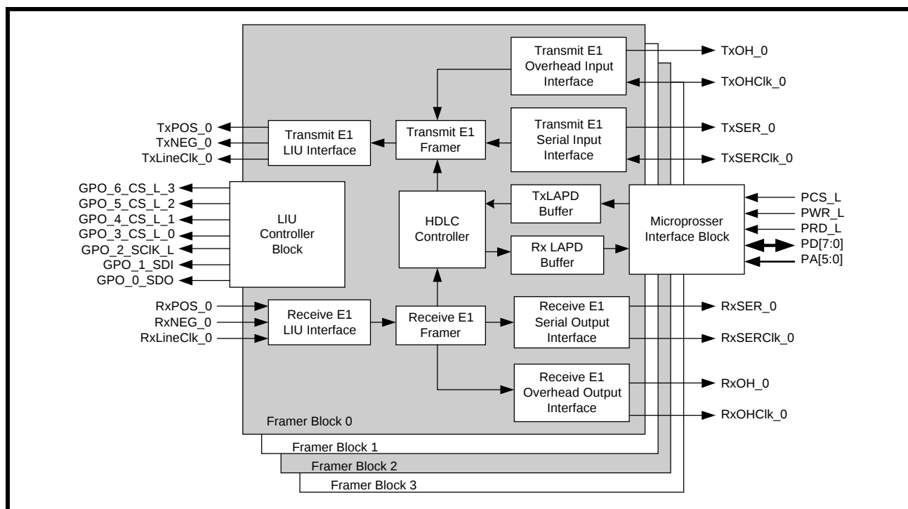
FIGURE 1. BLOCK DIAGRAM OF THE XRT84V24
