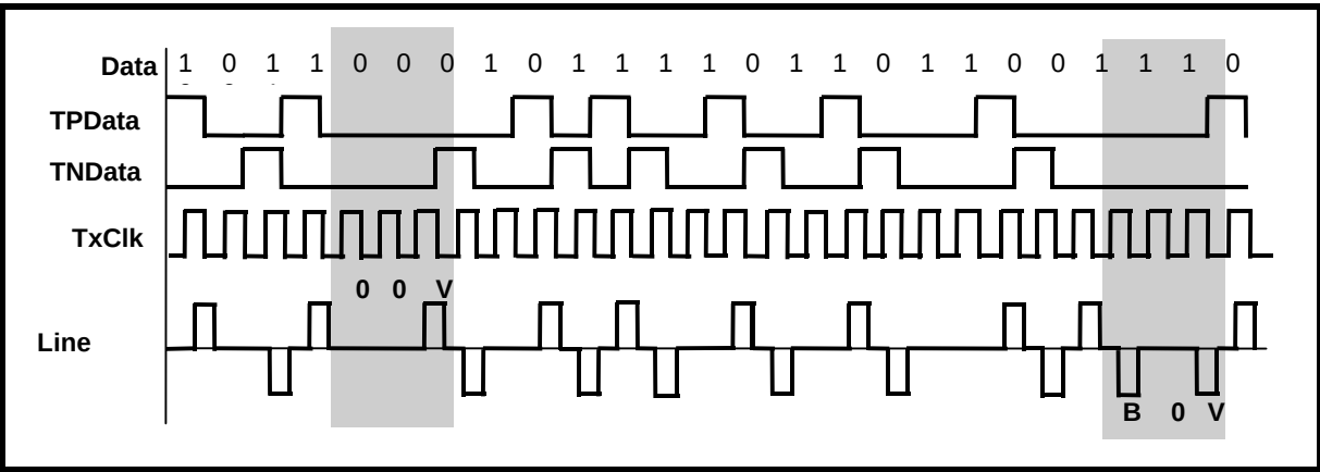
FIGURE 10. AN EXAMPLE OF B3ZS ENCODING
