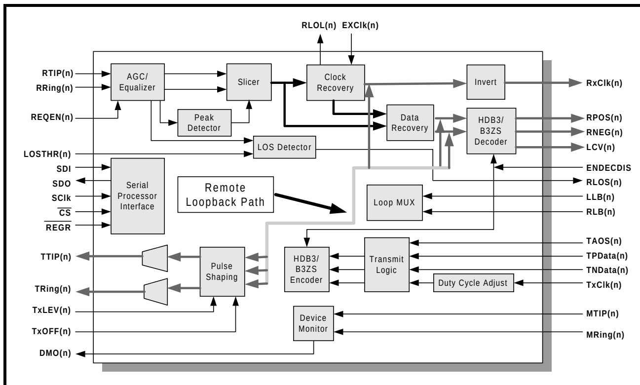
FIGURE 29. ILLUSTRATION OF THE "REMOTE LOOP-BACK" PATH, WITHIN A TYPICAL CHANNEL(N) (OF THE XRT7302 DEVICE)
