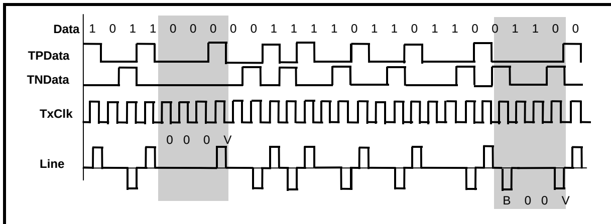
FIGURE 11. AN EXAMPLE OF HDB3 ENCODING
