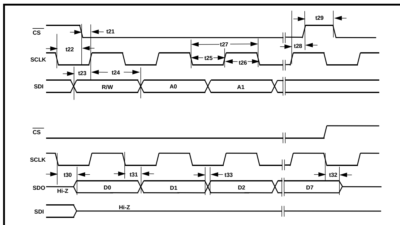
FIGURE 32. TIMING DIAGRAM FOR THE MICROPROCESSOR SERIAL INTERFACE
