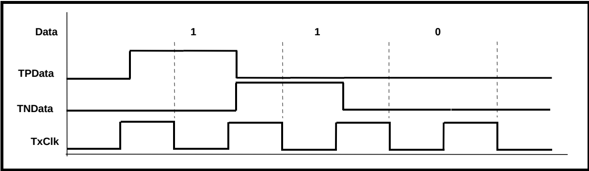
FIGURE 8. ILLUSTRATION ON HOW THE XRT7302 DEVICE SAMPLES THE DATA ON THE TPDATA AND TNDA INPUT PINS
