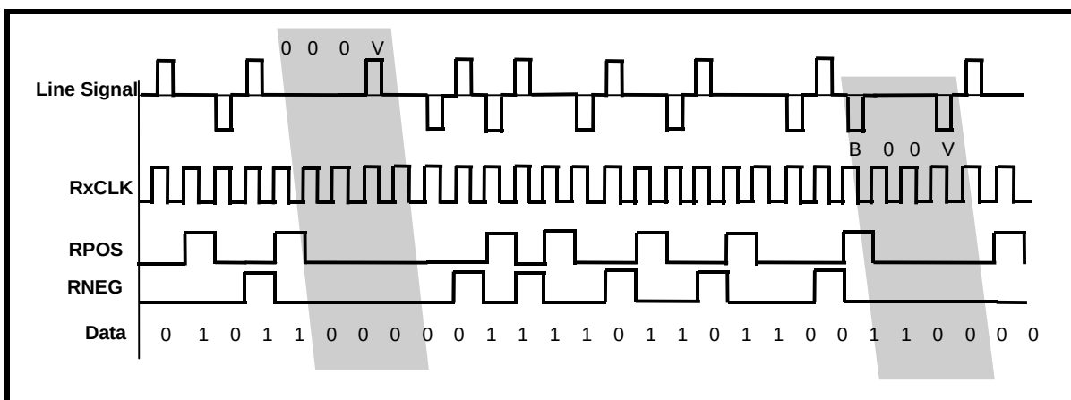
FIGURE 19. AN EXAMPLE OF HDB3 DECODING
