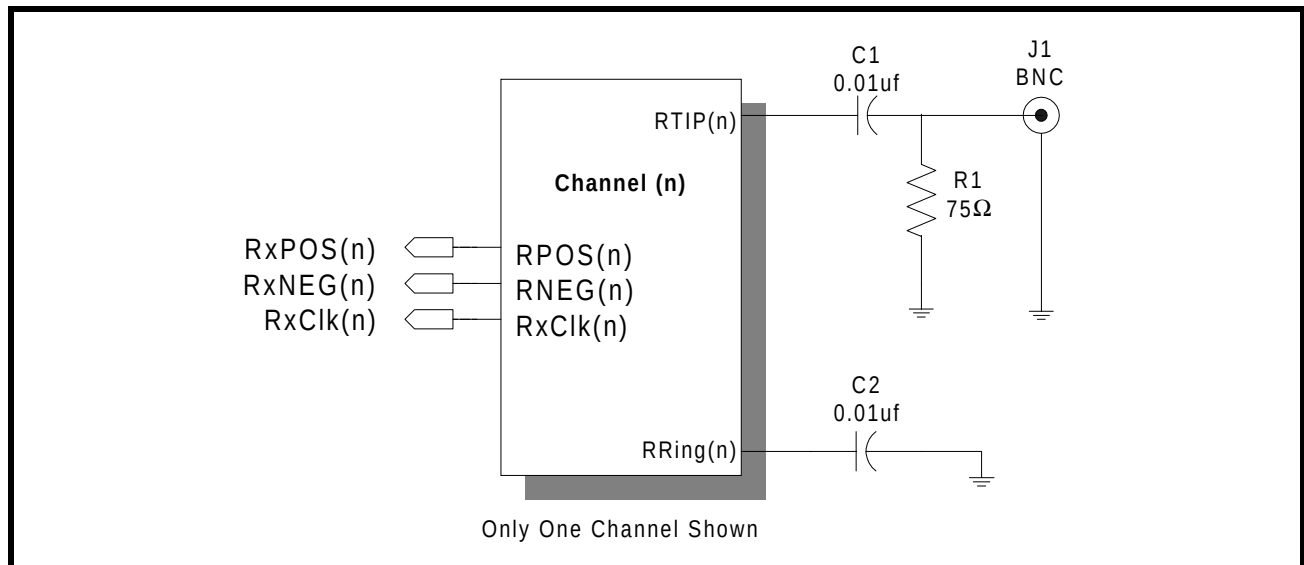
FIGURE 16. RECOMMENDED SCHEMATIC FOR INTERFACING THE RECEIVE SECTION OF THE XRT7302 DEVICE TO THE LINE (CAPACITIVE-COUPLING) - (TYPICAL CHANNEL SHOWN)
