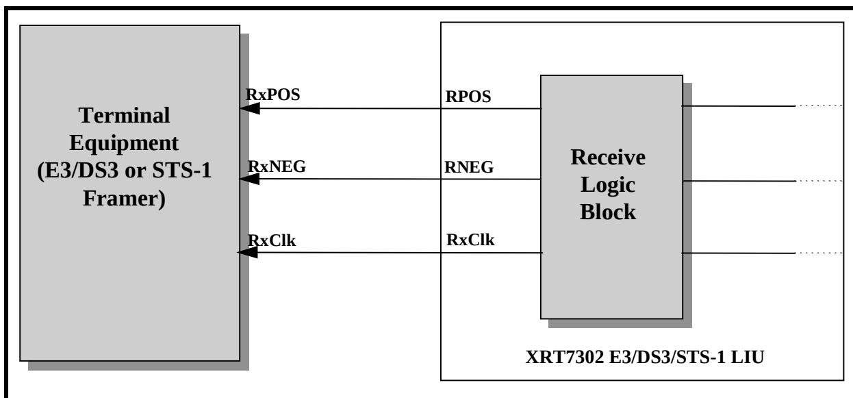
FIGURE 22. ILLUSTRATION OF THE TYPICAL INTERFACE FOR THE TRANSMISSION OF DATA IN A DUAL-RAIL FORMAT, FROM THE "RECEIVE SECTION" OF THE XRT7302 DEVICE TO THE RECEIVING TERMINAL EQUIPMENT
