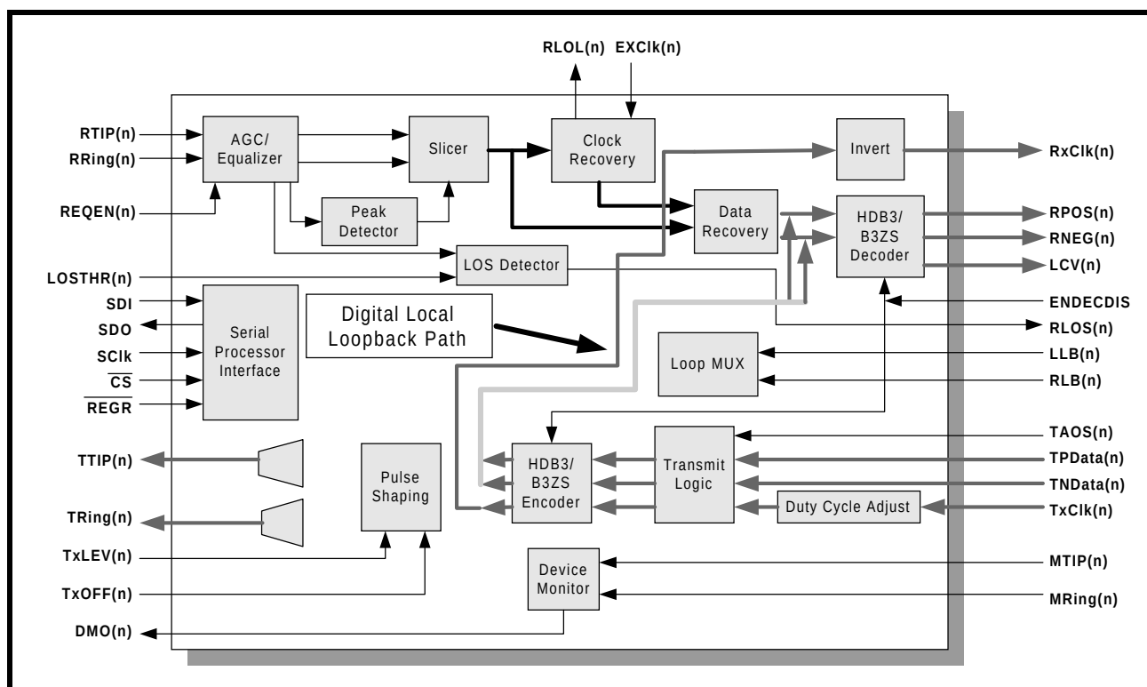
FIGURE 28. ILLUSTRATION OF THE "DIGITAL LOCAL LOOP-BACK" PATH IN A TYPICAL CHANNEL(N) (OF THE XRT7302 DEVICE)
