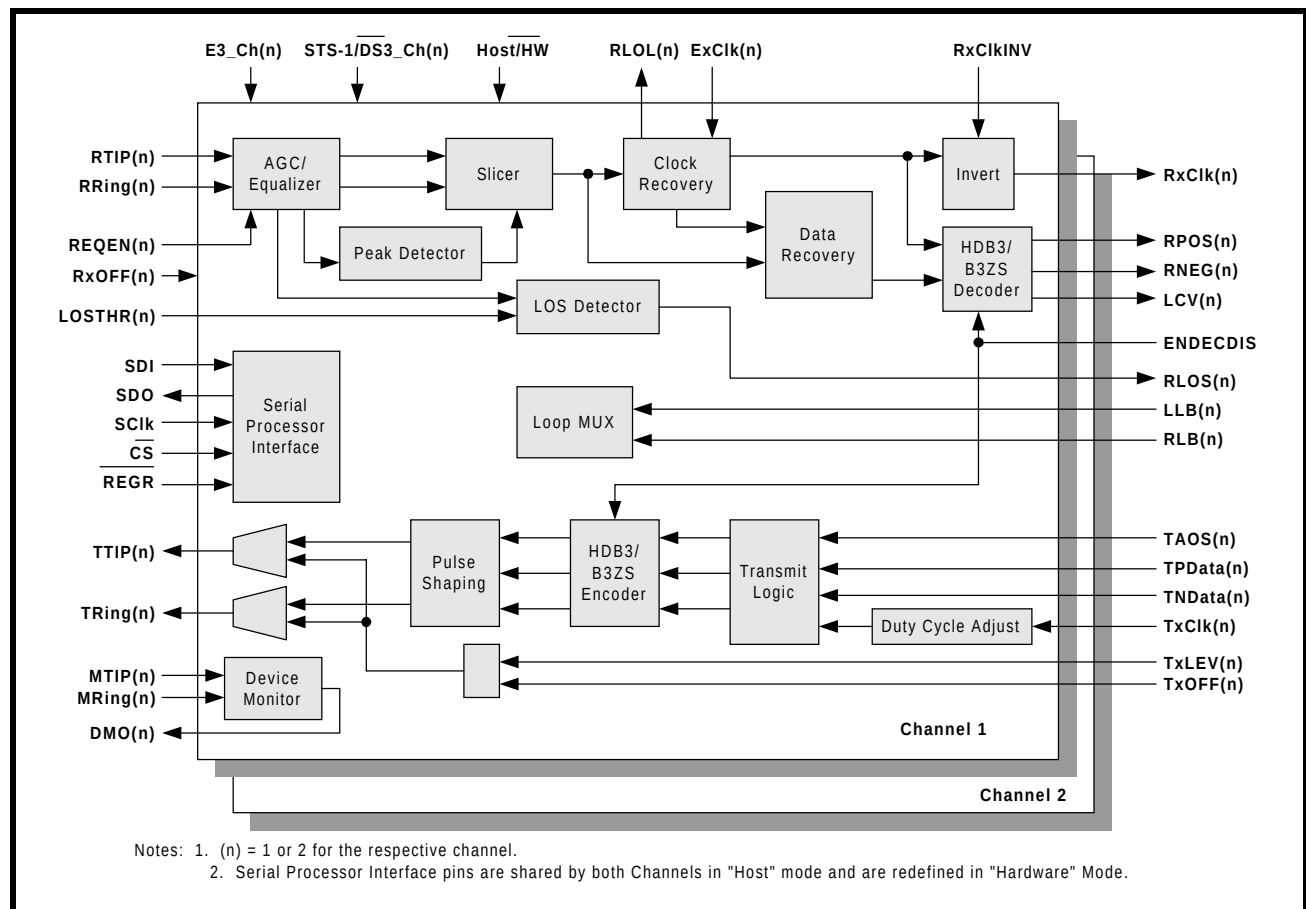
FIGURE 6. FUNCTIONAL BLOCK DIAGRAM OF THE XRT7302 DEVICE
