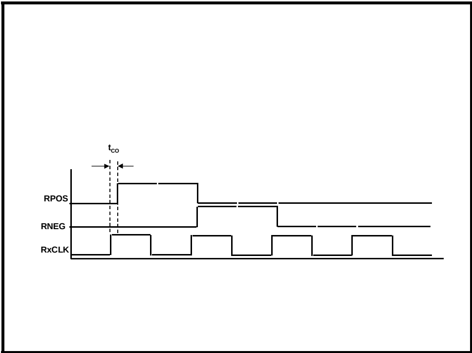
FIGURE 3. TIMING DIAGRAM OF THE RECEIVE TERMINAL OUTPUT INTERFACE
