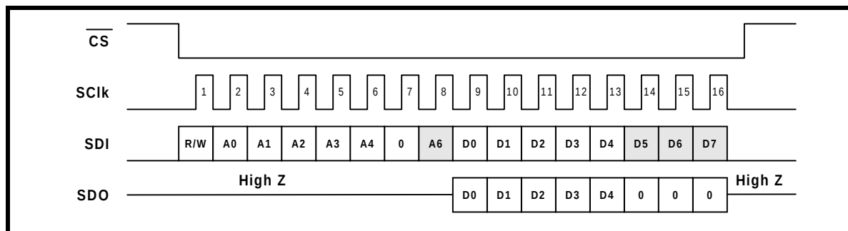
FIGURE 32. TIMING DIAGRAM FOR THE MICROPROCESSOR SERIAL INTERFACE
