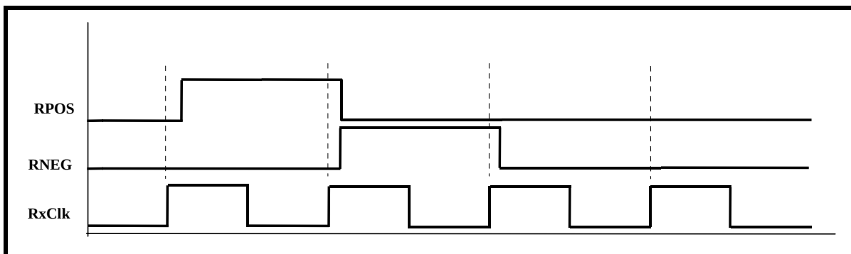
FIGURE 23. ILLUSTRATION ON HOW THE XRT7302 DEVICE OUTPUTS DATA ON THE RPOS AND RNEG OUTPUT PINS
