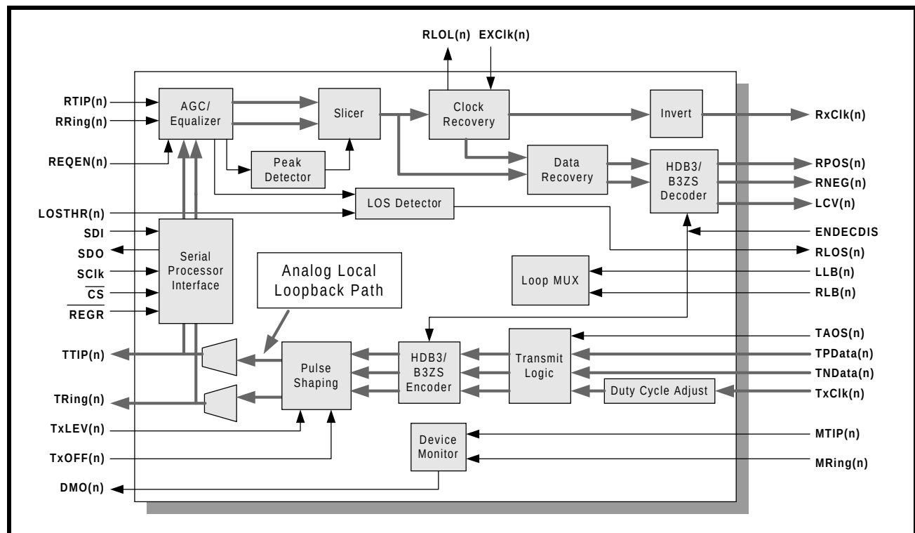
FIGURE 27. ILLUSTRATION OF A TYPICAL CHANNEL(N) (WITHIN THE XRT7302 DEVICE) OPERATING IN THE ANALOG LOCAL LOOP-BACK MODE
