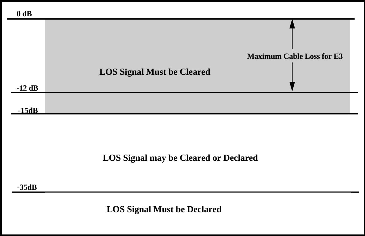
FIGURE 20. ILLUSTRATION OF THE SIGNAL LEVELS THAT THE XRT7302 DEVICE WILL DECLARE AND CLEAR LOS
