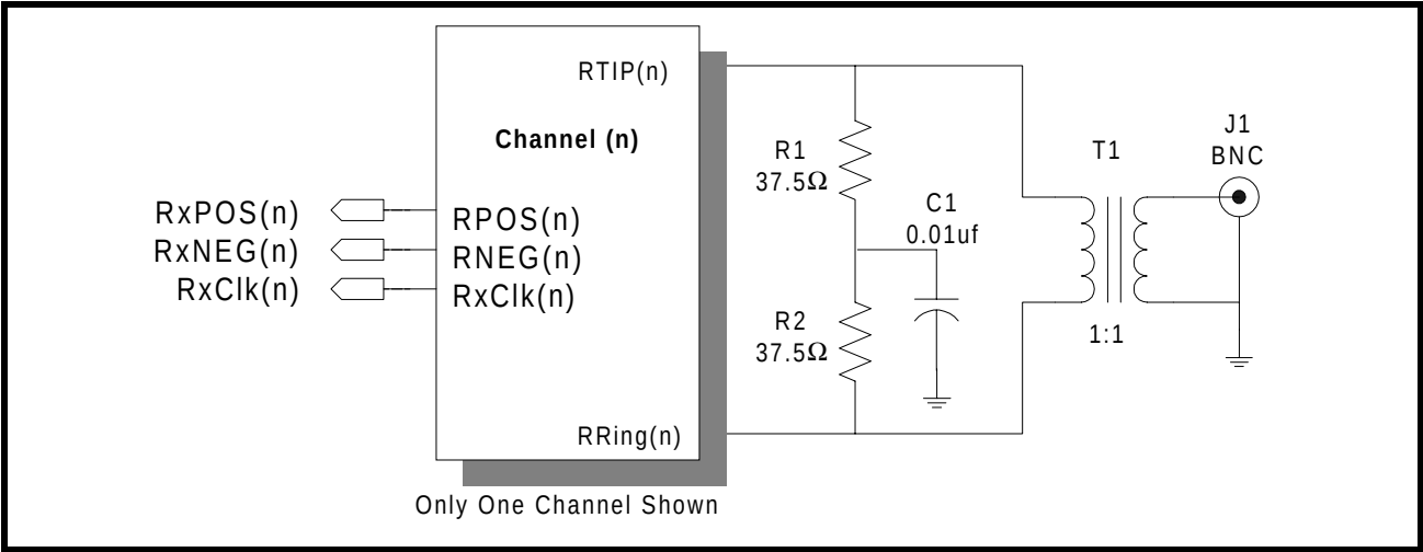
FIGURE 15. RECOMMENDED SCHEMATIC FOR INTERFACING THE RECEIVE SECTION OF THE XRT7302 DEVICE TO THE LINE (TRANSFORMER-COUPLING)
