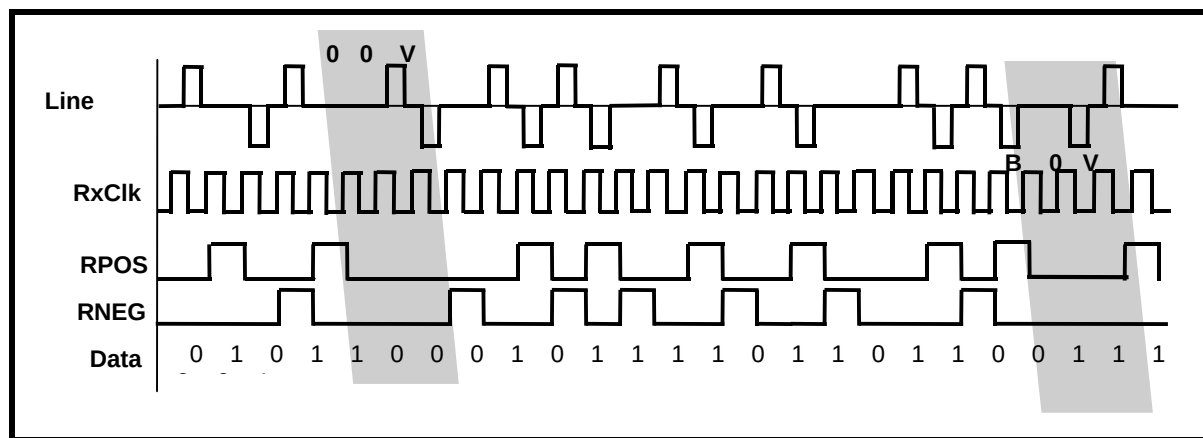
FIGURE 18. AN EXAMPLE OF B3ZS DECODING
