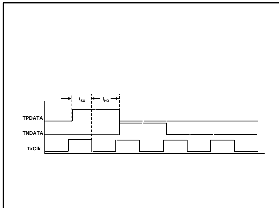
FIGURE 2. TIMING DIAGRAM OF THE TRANSMIT TERMINAL INPUT INTERFACE
