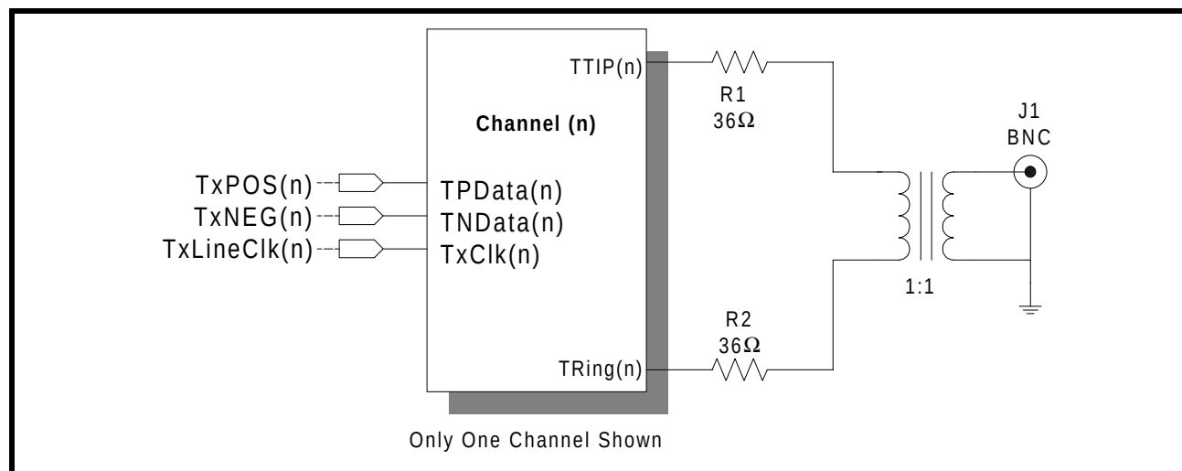
FIGURE 14. RECOMMENDED SCHEMATIC FOR INTERFACING THE TRANSMIT SECTION OF THE XRT7302 DEVICE TO THE LINE
