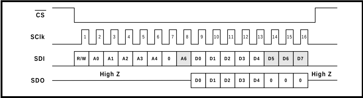
FIGURE 4. MICROPROCESSOR SERIAL INTERFACE DATA STRUCTURE
