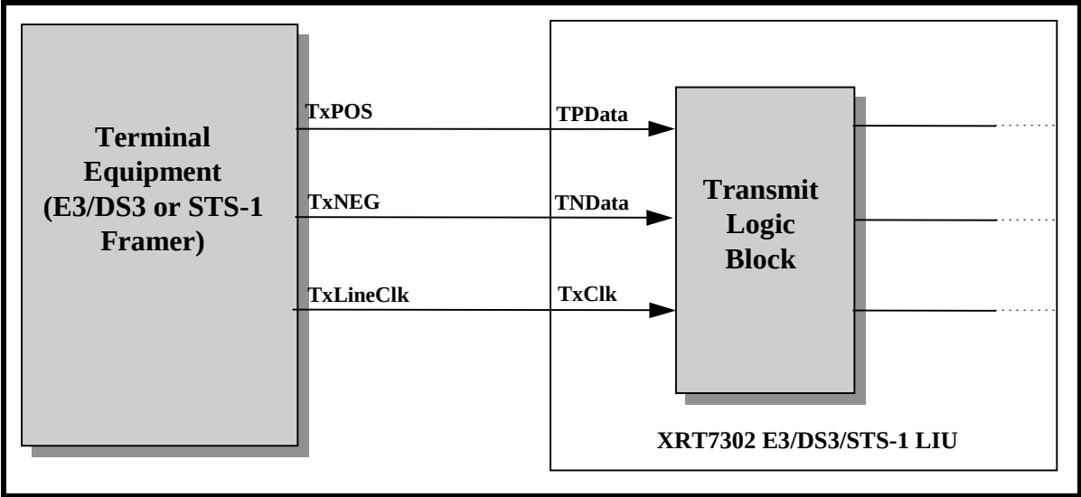
FIGURE 7. ILLUSTRATION OF THE TYPICAL INTERFACE FOR THE TRANSMISSION OF DATA IN A DUAL RAIL FORMAT, FROM THE "TRANSMITTING" TERMINAL EQUIPMENT TO THE "TRANSMIT SECTION" OF A CHANNEL WITHIN THE XRT7302 DEVICE
