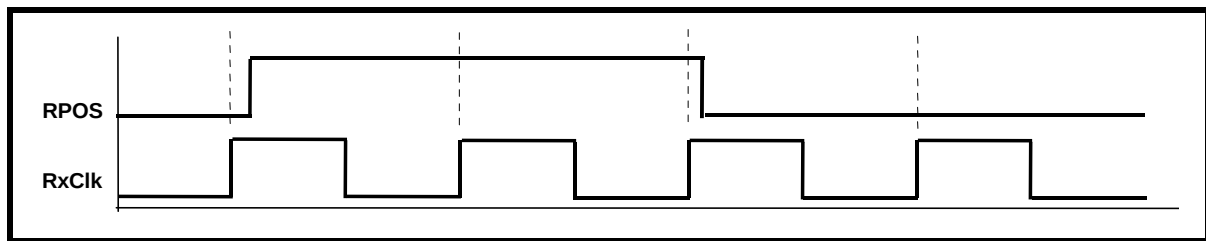
FIGURE 26. ILLUSTRATION OF THE BEHAVIOR OF THE RPOS AND RxCLK OUTPUT SIGNALS, WHILE THE XRT7302 DEVICE IS TRANSMITTING "SINGLE-RAIL" DATA TO THE RECEIVING TERMINAL EQUIPMENT
