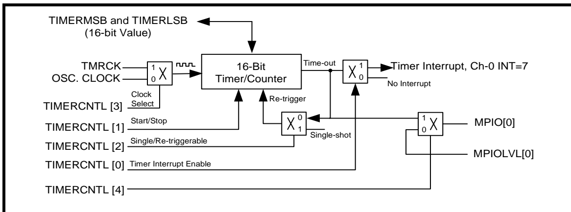
FIGURE 5. TIMER/COUNTER CIRCUIT.
