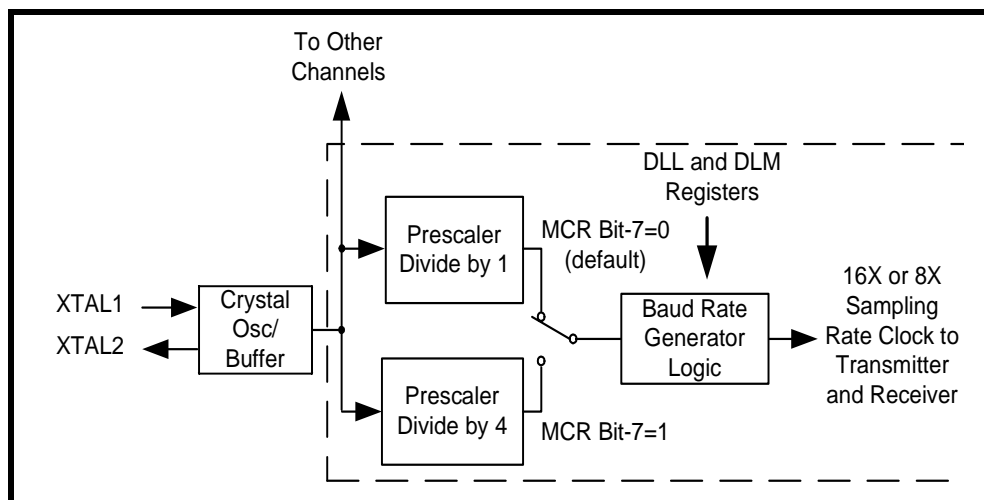
FIGURE 8. BAUD RATE GENERATOR
