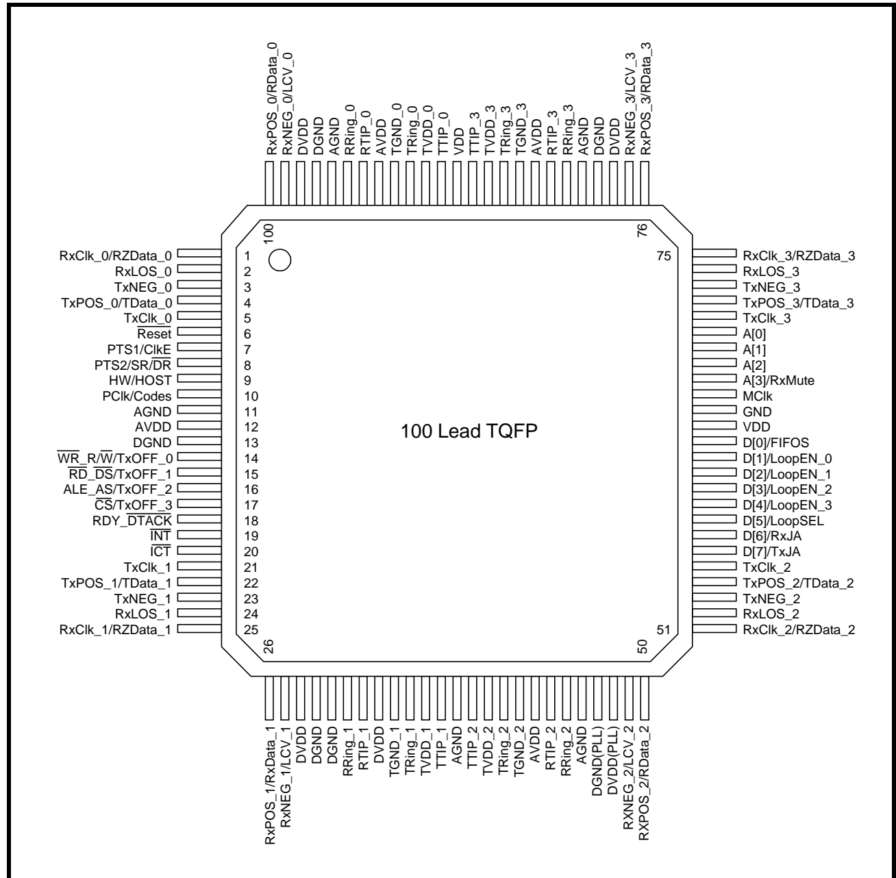
FIGURE 3. PIN OUT OF THE XRT82L24
