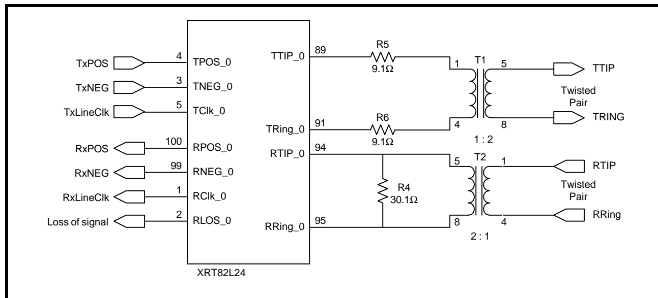
FIGURE 13. XRT 82L24 CHANNEL 1 - E1 120 \Omega BALANCED APPLICATION
