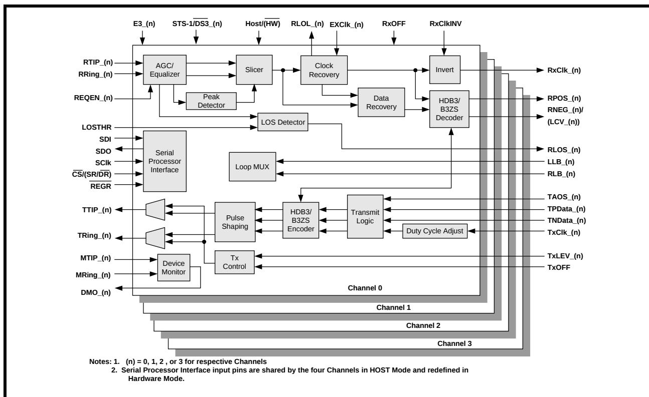
FIGURE 1. XRT73L04A BLOCK DIAGRAM
