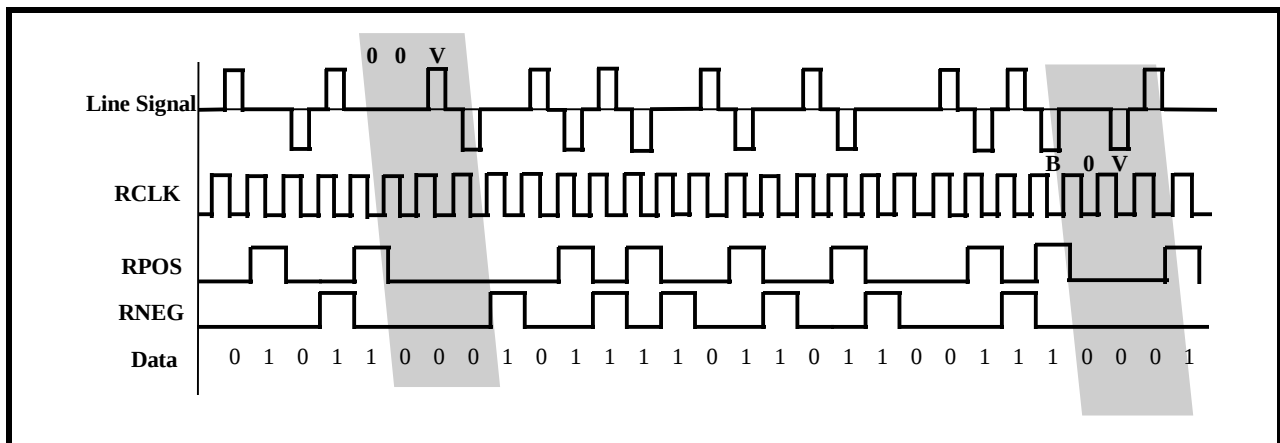
FIGURE 25. AN EXAMPLE OF B3ZS DECODING
