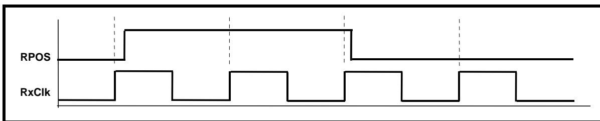
FIGURE 33. THE BEHAVIOR OF THE RPOS AND RxClk OUTPUT SIGNALS WHILE THE XRT73L04 IS TRANSMITTING SINGLE-RAIL DATA TO THE RECEIVING TERMINAL EQUIPMENT
