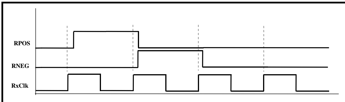
FIGURE 30. HOW THE XRT73L04 OUTPUTS DATA ON THE RPOS AND RNEG OUTPUT PINS
