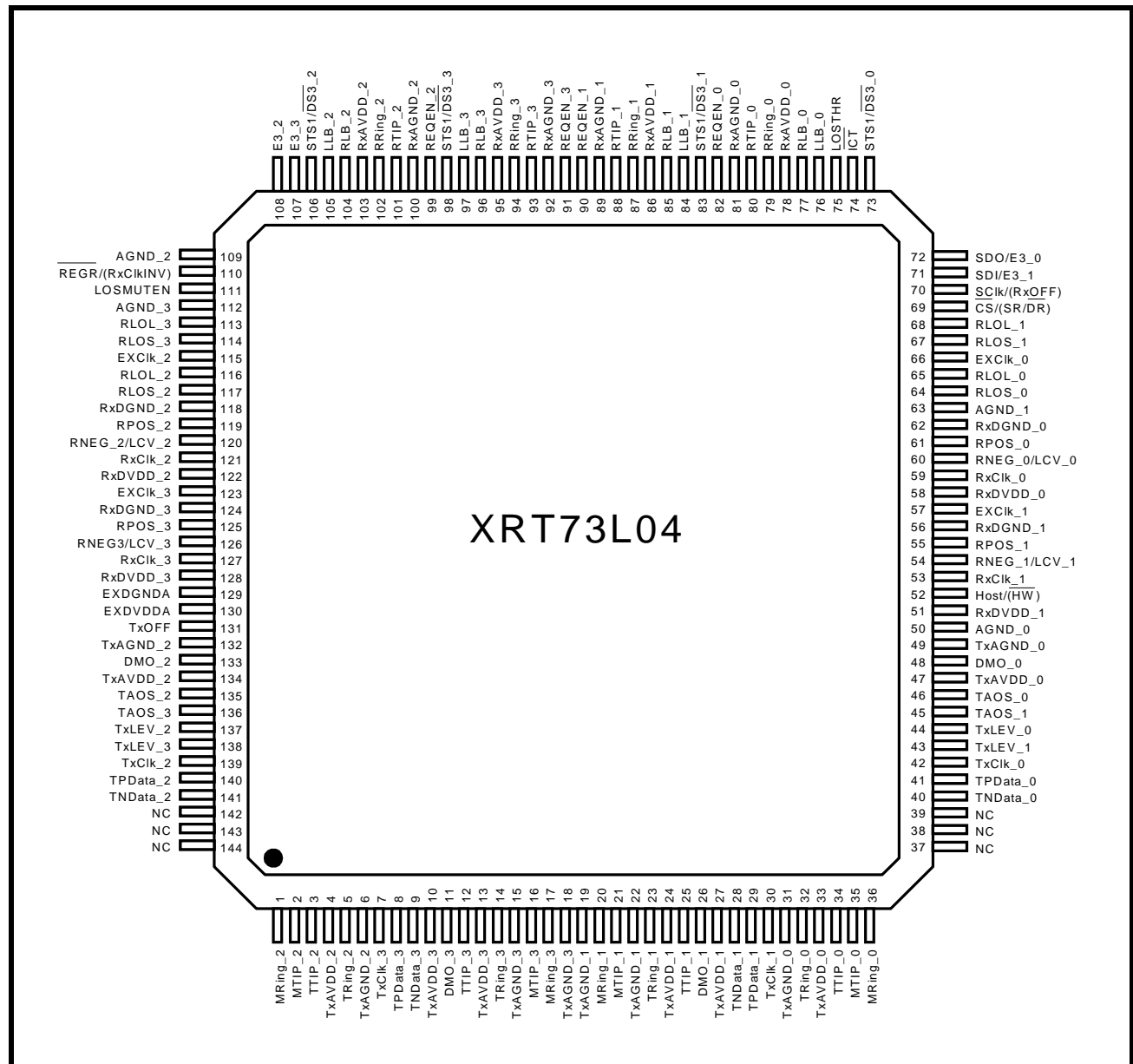
FIGURE 4. PIN OUT OF THE XRT73L04 IN THE 144 PIN TQFP PACKAGE
