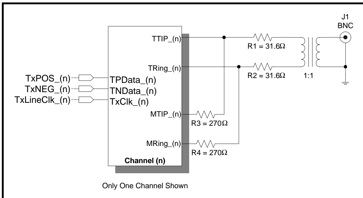
FIGURE 37. THE XRT73L04 EMPLOYING THE TRANSMIT DRIVE MONITOR FEATURES
