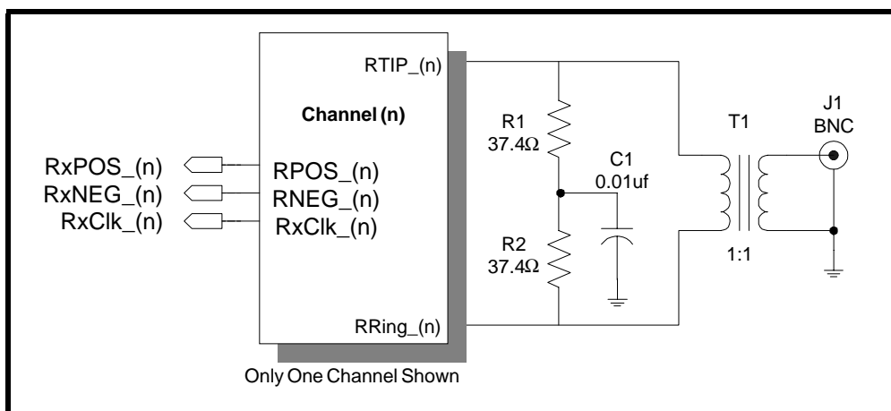
FIGURE 22. RECOMMENDED SCHEMATIC FOR INTERFACING THE RECEIVE SECTION OF THE XRT73L04 TO THE LINE (TRANSFORMER-COUPLING)
