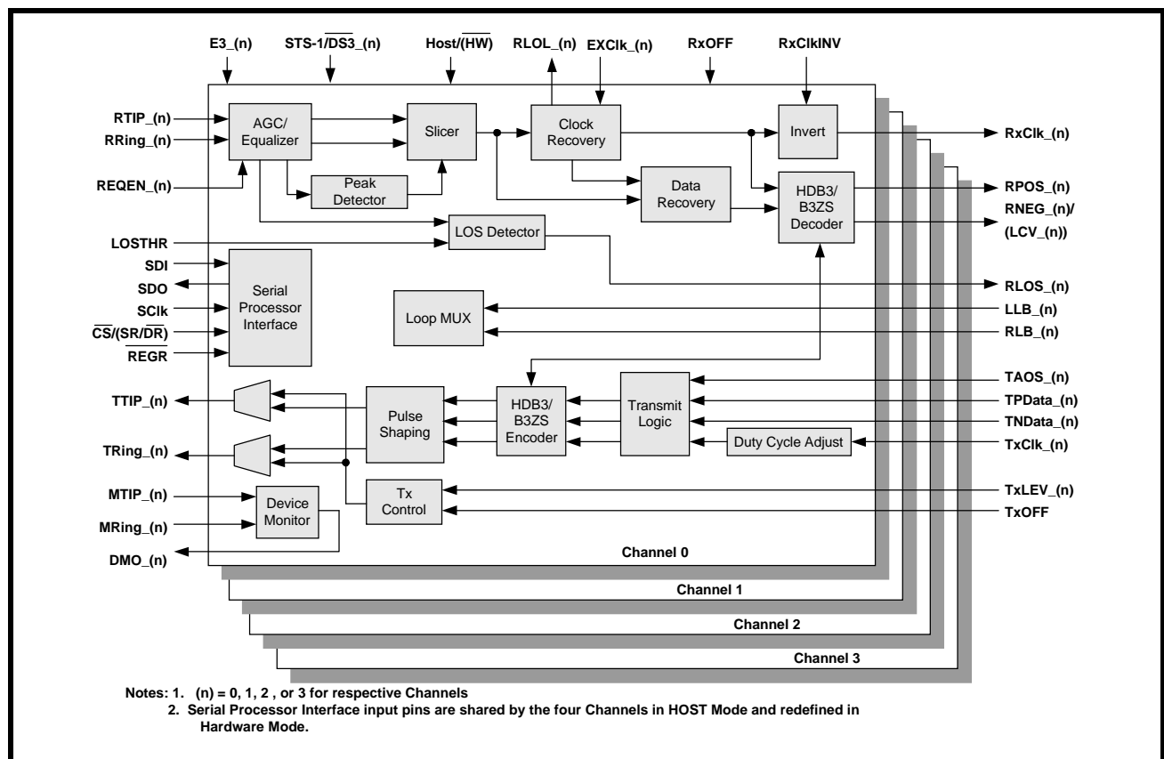
FIGURE 1. XRT73L04 BLOCK DIAGRAM
