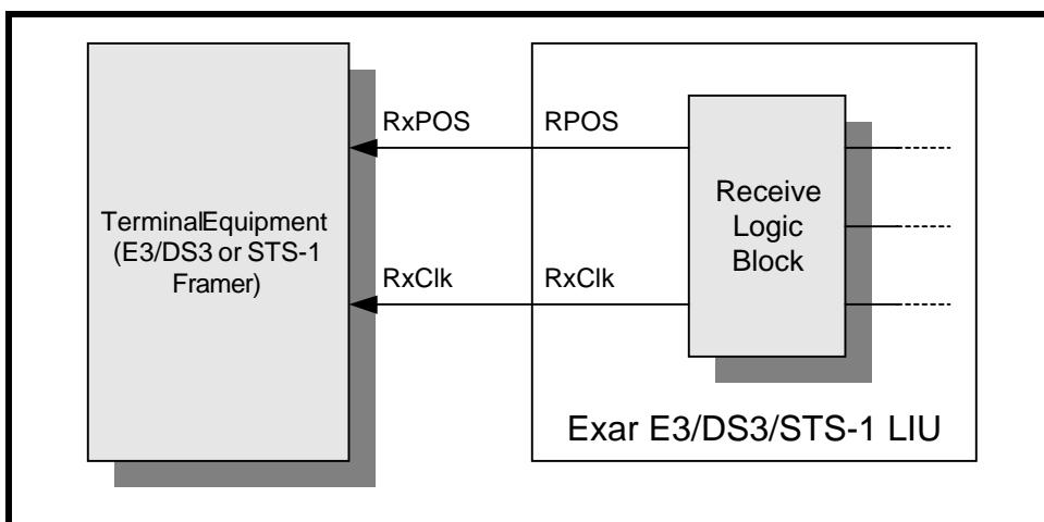
FIGURE 32. THE TYPICAL INTERFACE FOR THE TRANSMISSION OF DATA IN A SINGLE-RAIL FORMAT FROM THE RECEIVE SECTION OF THE XRT73L04 TO THE RECEIVING TERMINAL EQUIPMENT
