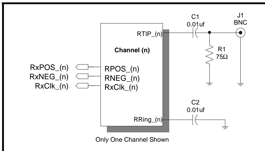
FIGURE 23. RECOMMENDED SCHEMATIC FOR INTERFACING THE RECEIVE SECTION OF THE XRT73L04 TO THE LINE (CAPACITIVE-COUPLING)
