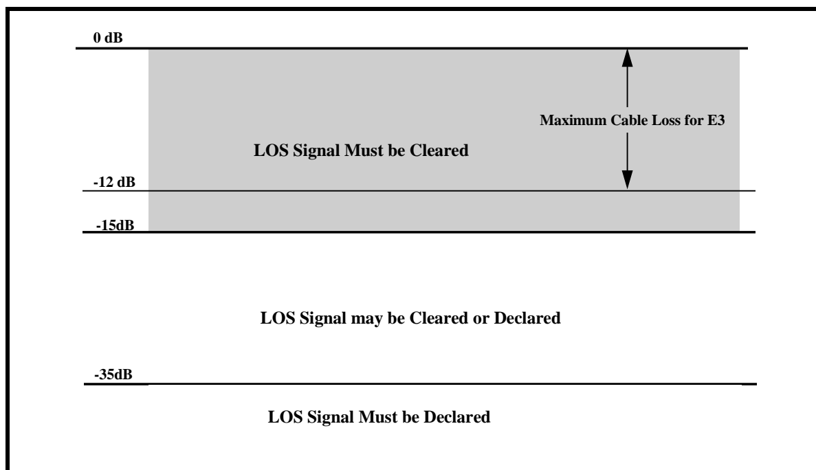
FIGURE 27. THE SIGNAL LEVELS THAT THE XRT73L04 DECLARES AND CLEARS LOS
