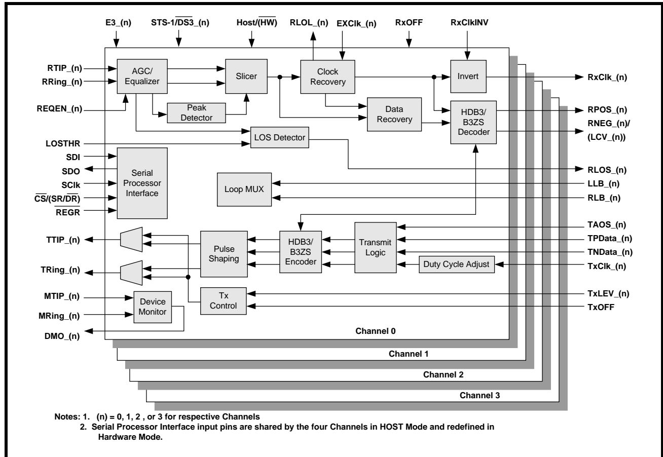
FIGURE 13. FUNCTIONAL BLOCK DIAGRAM OF THE XRT73L04
