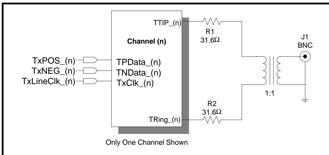
FIGURE 21. RECOMMENDED SCHEMATIC FOR INTERFACING THE TRANSMIT SECTION OF THE XRT73L04 TO THE LINE
