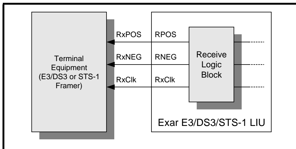
FIGURE 29. THE TYPICAL INTERFACE FOR THE TRANSMISSION OF DATA IN A DUAL-RAIL FORMAT, FROM THE RECEIVE SECTION OF THE XRT73L04 TO THE RECEIVING TERMINAL EQUIPMENT
