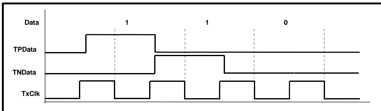
FIGURE 15. THE XRT73L04 SAMPLES THE DATA ON THE TPDATA AND TNDATA INPUT PINS
