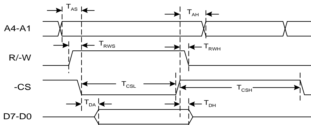
Read Cycle Timing
