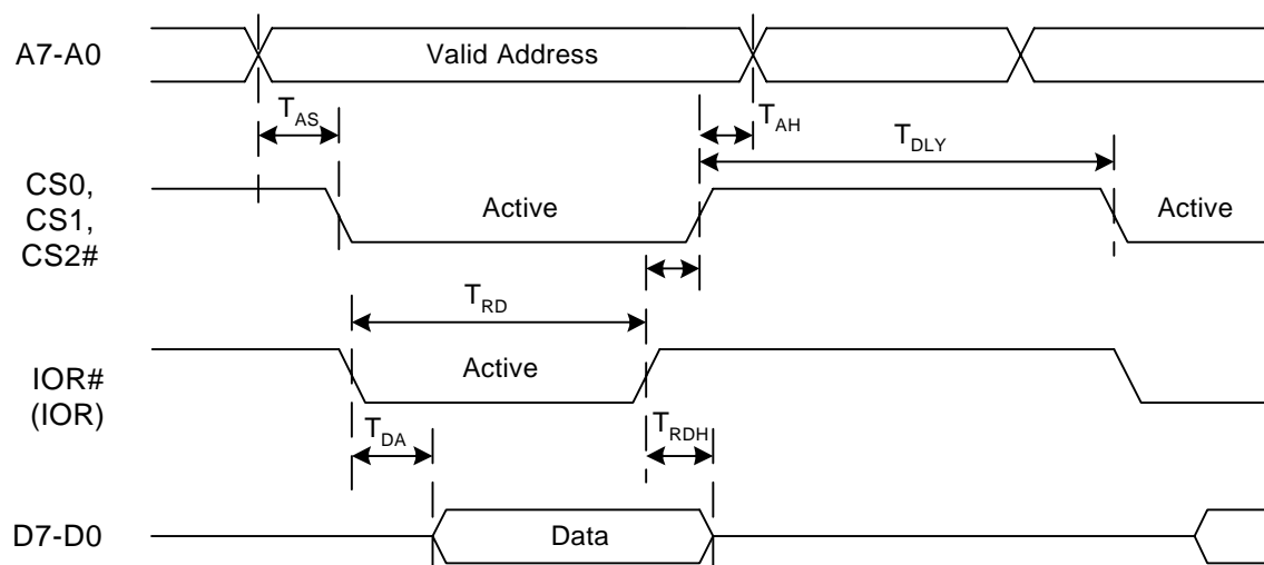
FIGURE 16. INTEL DATA BUS READ AND WRITE TIMING
