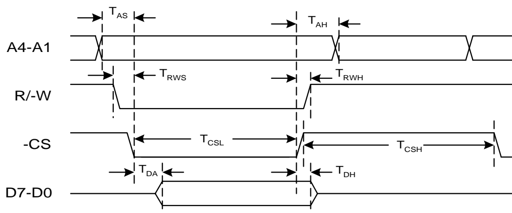
Write Cycle Timing
