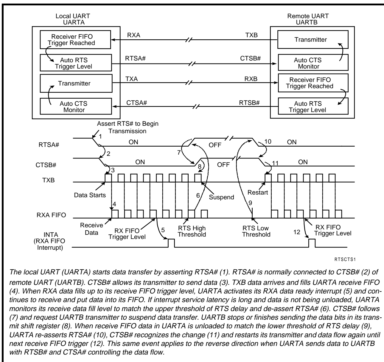
FIGURE 9. AUTO RTS AND CTS FLOW CONTROL OPERATION
