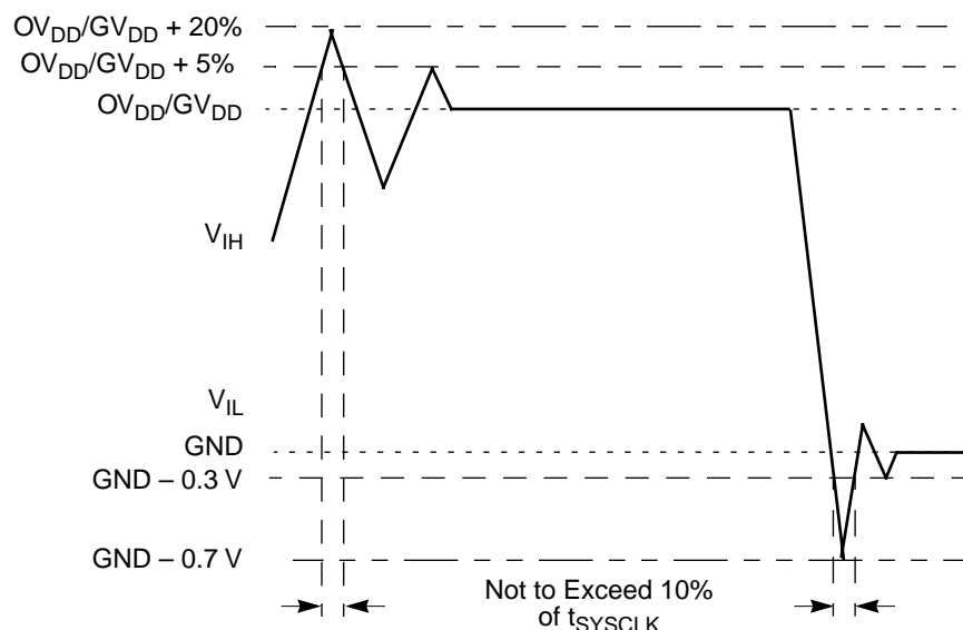
Figure 2. Overshoot/Undershoot Voltage
