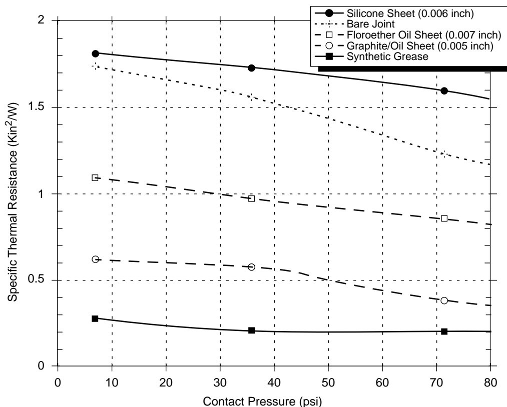
Figure 27. Thermal Performance of Select Thermal Interface Material
