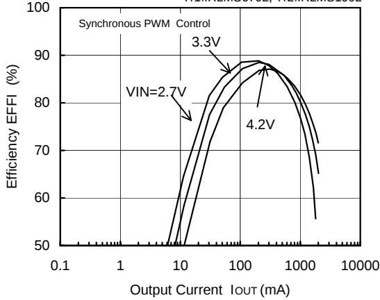
FOSC=300kHz, V_{OUT}=5.0V
