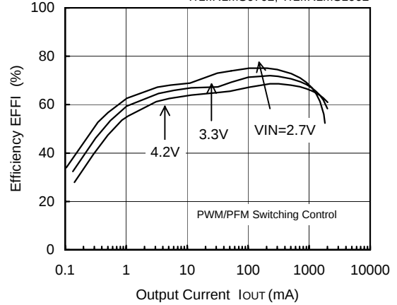
FOSC=300kHz, V_{OUT}=5.0V
