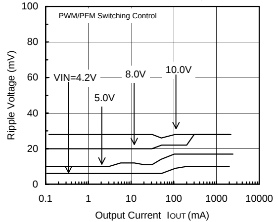
FOSC=300kHz, V_{OUT}=5.0V
