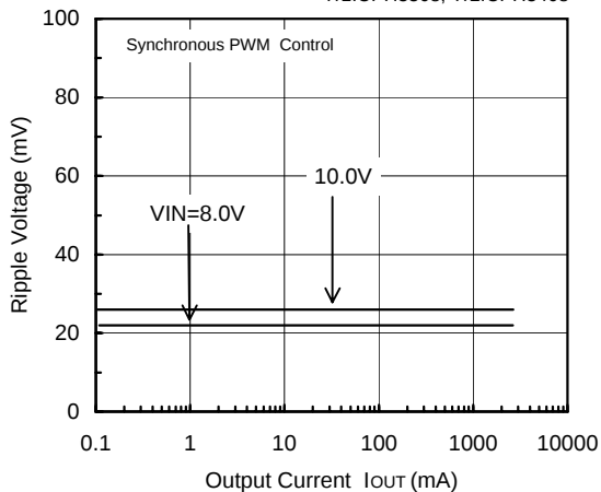
FOSC=300kHz, V_{OUT}=5.0V
