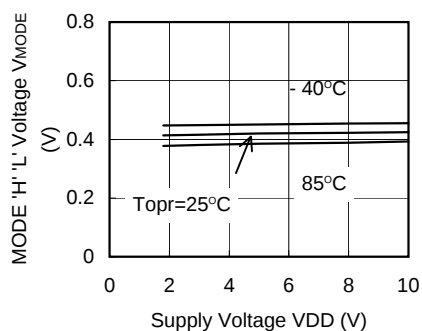
(12) MODE 'H' 'L' Voltage vs. Supply Voltage
