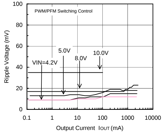
FOSC=300kHz, V_{OUT}=3.3V
