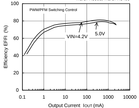
FOSC=180kHz, V_{OUT}=1.8V
