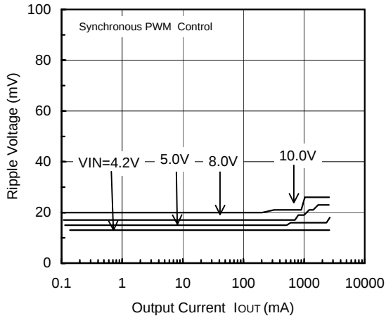
FOSC=300kHz, V_{OUT}=3.3V
