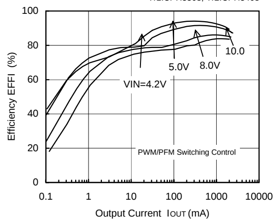
FOSC=300kHz, V_{OUT}=5.0V
