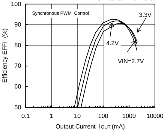
FOSC=180kHz, V_{OUT}=1.2V
