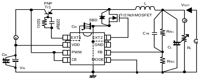
Circuit 3
