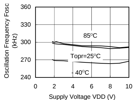
(13) Oscillation Frequency vs. Supply Voltage
