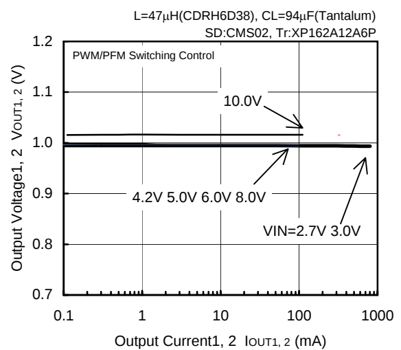
FOSC=180kHz, V OUT1, 2 =1.0V
