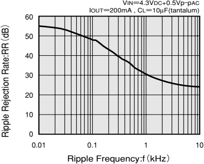
XC62EP3302 (3.3V)
