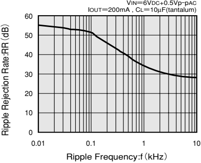
XC62EP5002 (5V)
