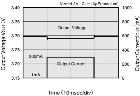
XC62EP3302 (3.3V)
