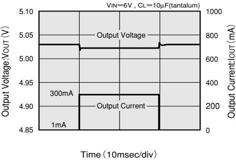
XC62EP5002 (5V)
