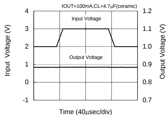
XC6205x092
