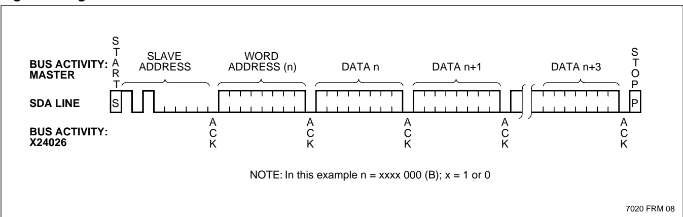
Figure 6. Page Write
