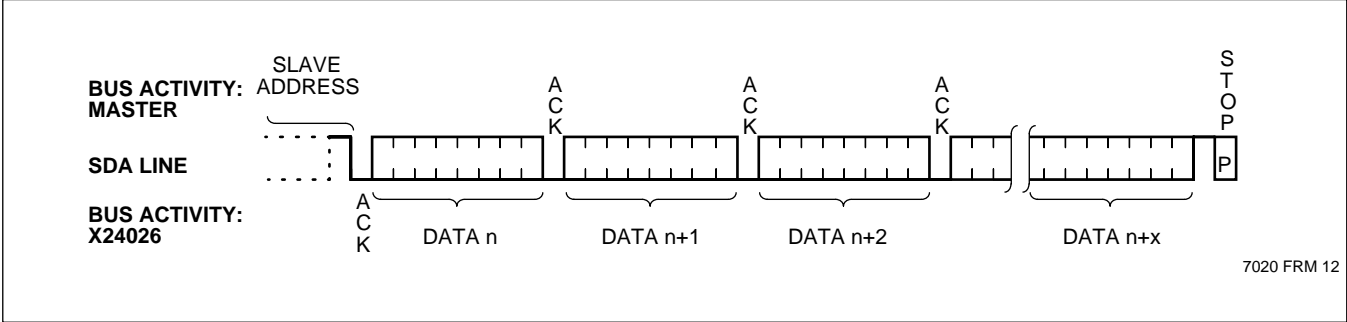
Figure 9. Sequential Read
