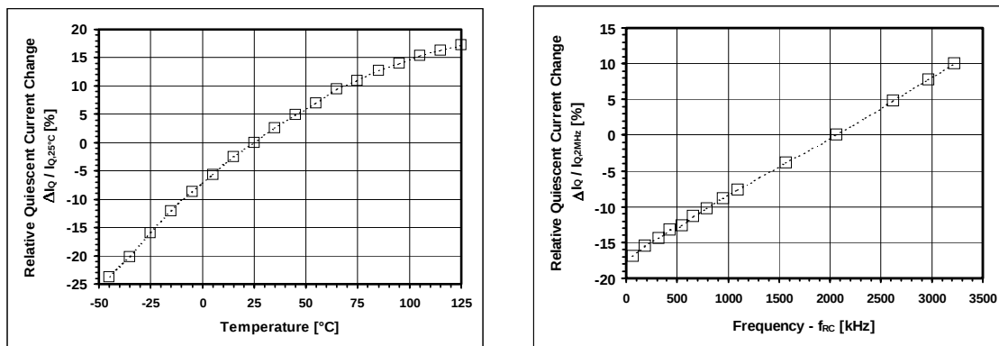
Figure 8.5: Relative change in quiescent current consumption vs. temperature and clock speed clock
