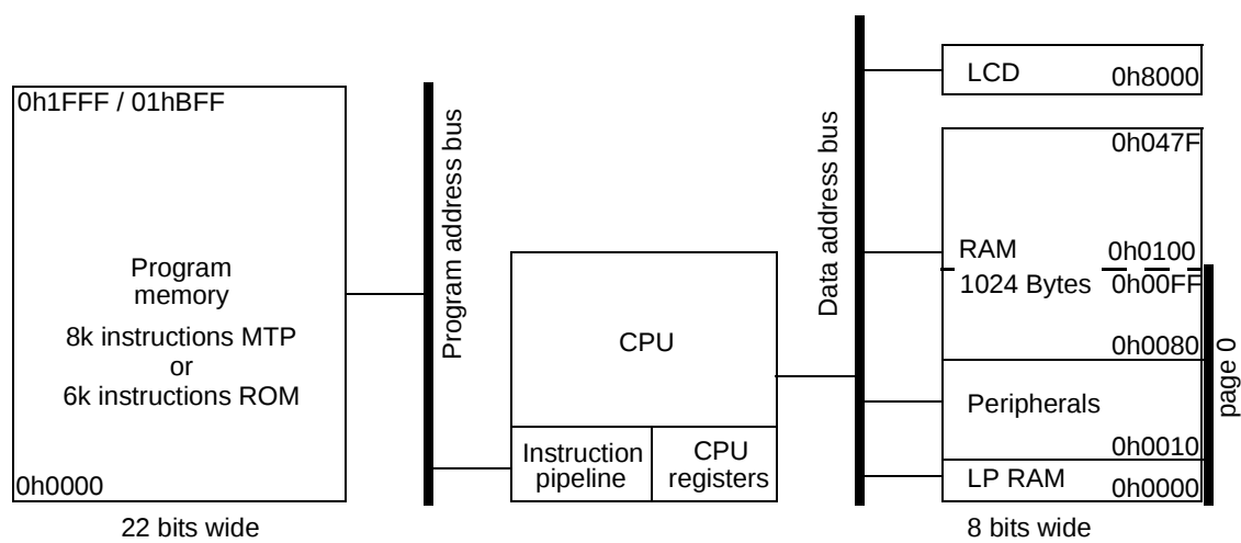
Figure 5.1: Memory organization
