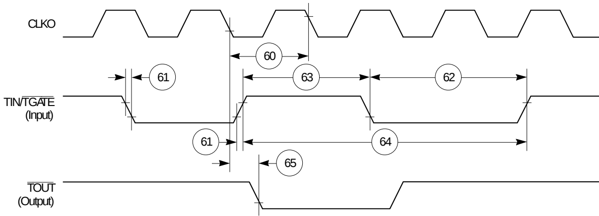
Figure 50. CPM General-Purpose Timers Timing Diagram
