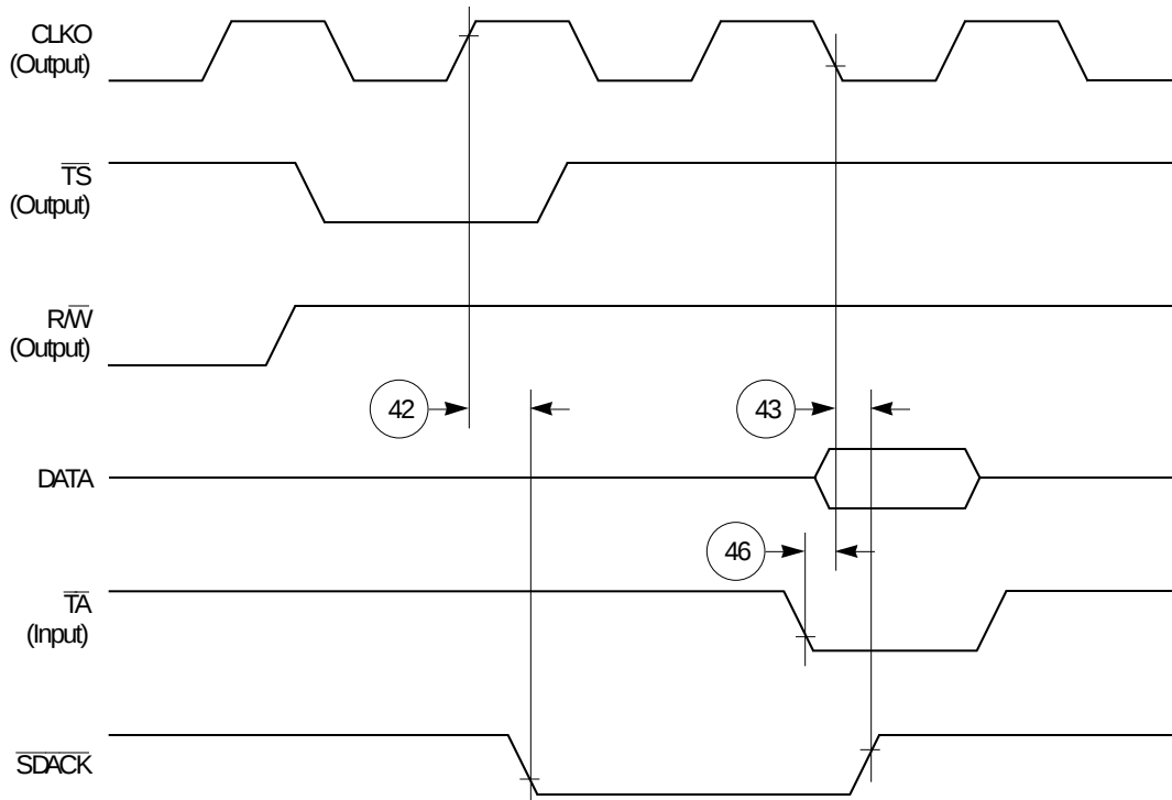
Figure 46. \overline{SDACK} Timing Diagram—Peripheral Write, Externally-Generated \overline{TA}
