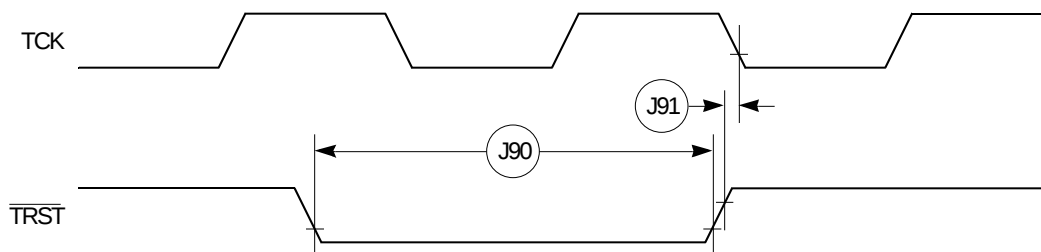
Figure 37. JTAG \overline{\text{TRST}} Timing Diagram
