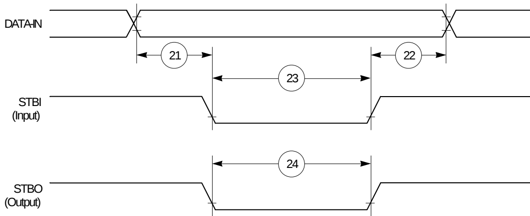
Figure 41. PIP Rx (Pulse Mode) Timing Diagram
