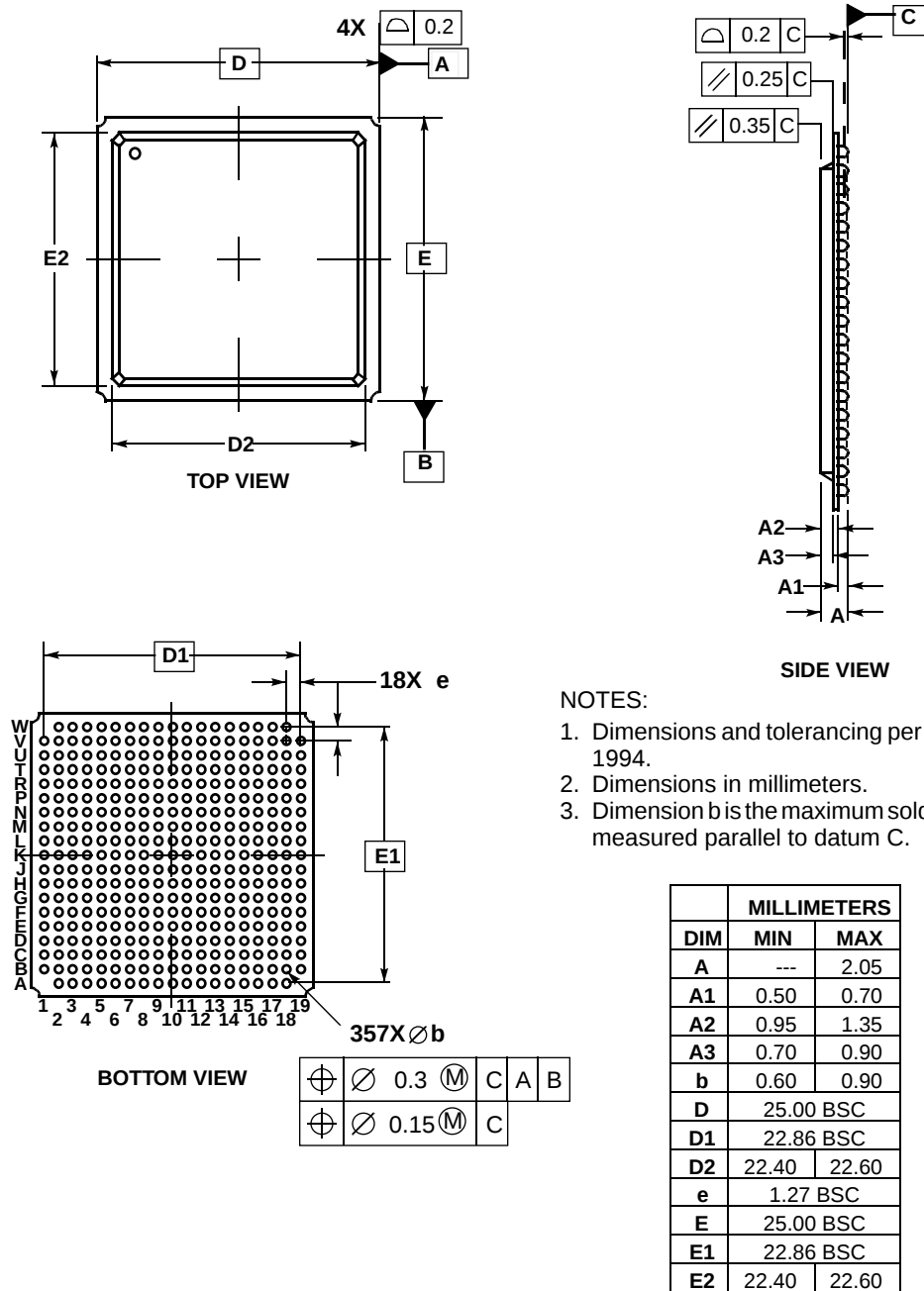
Figure 77. Mechanical Dimensions and Bottom Surface Nomenclature of the PBGA Package
