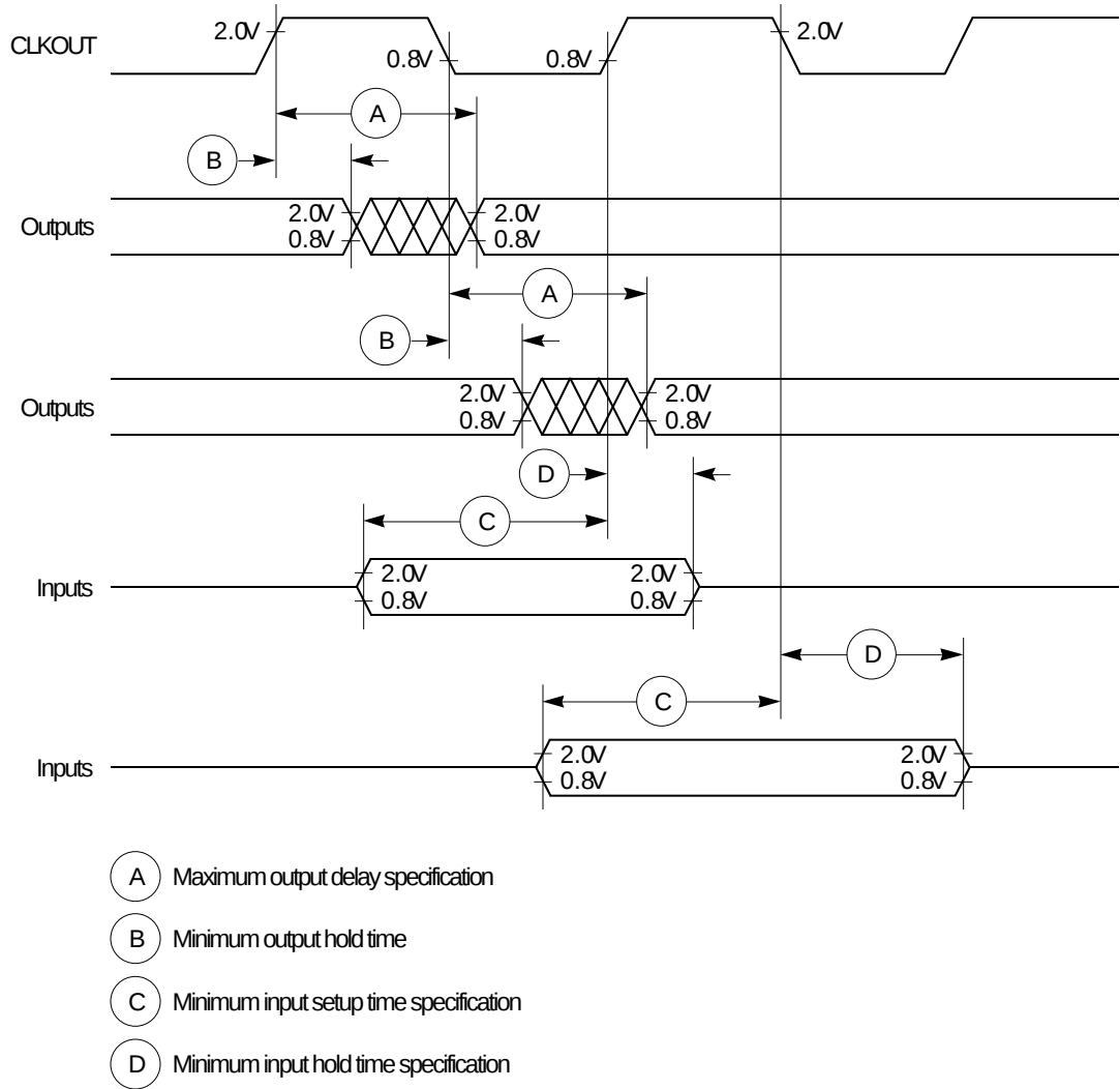
Figure 3. Control Timing
