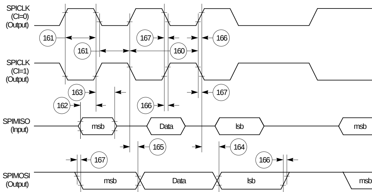
Figure 66. SPI Master (CP = 1) Timing Diagram
