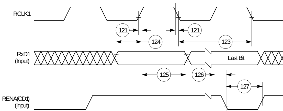
Figure 60. Ethernet Receive Timing Diagram
