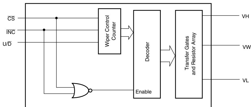
Figure 1. Functional Diagram
