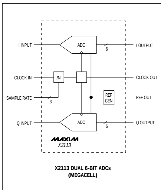
Block Diagram
