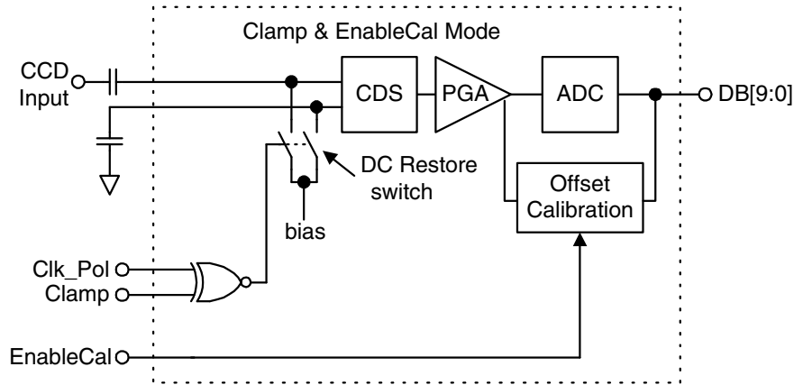
Figure 20. Clamp & Enable Cal Mode (XRD9853 Compatible), M1=1, M3=3
