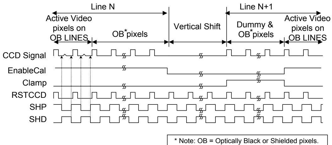
Figure 16. Frame Calibration Mode Timing, CLK_POL= High
