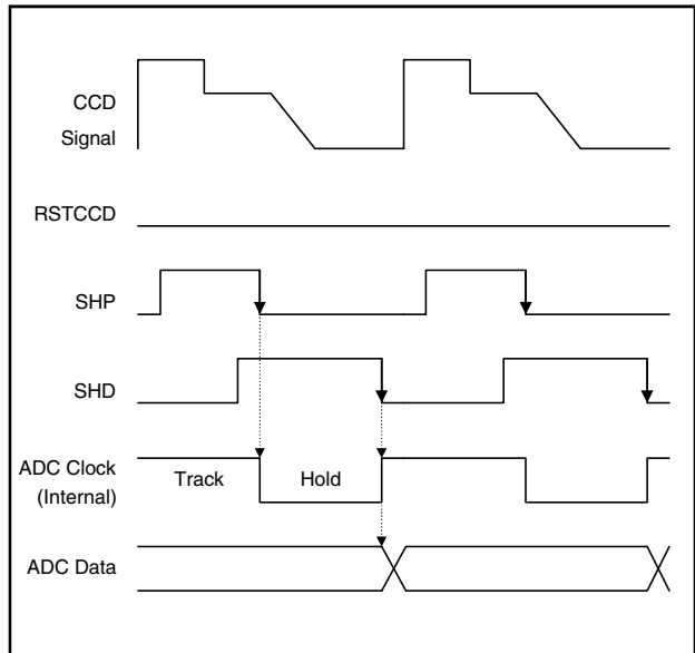
Figure 23. ADC Clock Generation, CLK_POL=1, M2=1
