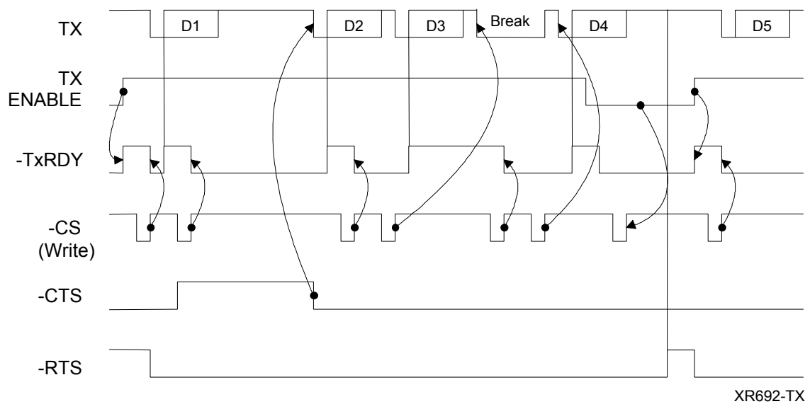
Figure 9: Transmit Timing
