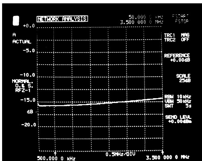
Figure 7. 120 \Omega Return Loss Measurement
