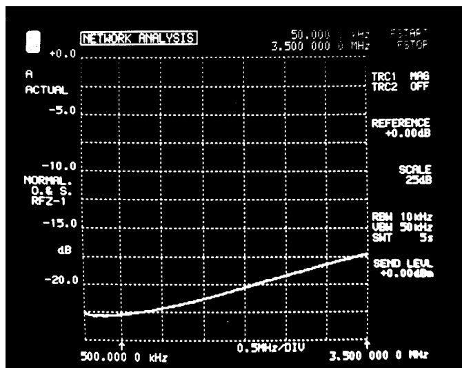
Figure 6. 75 \Omega Return Loss Measurement
