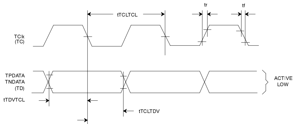
Figure 11. Transmit Timing
