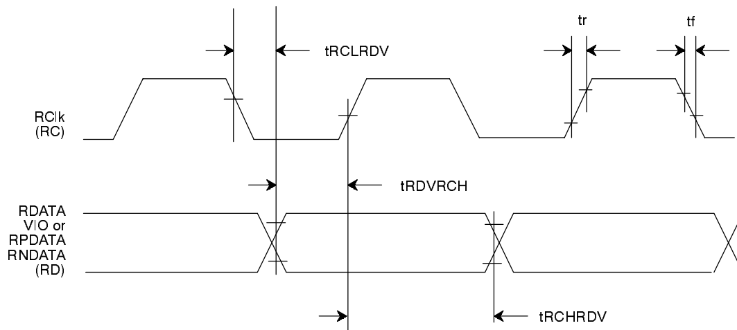
Figure 10. Receive Timing
