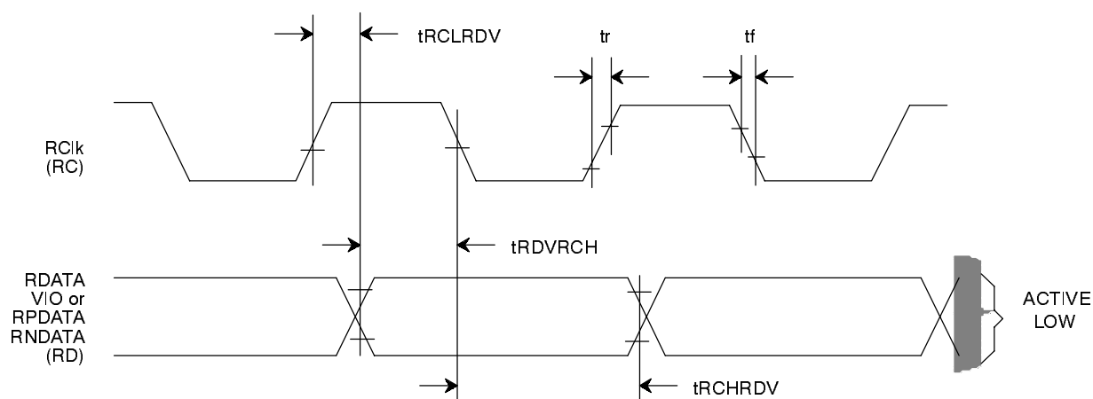
Figure 12. Receive Timing
