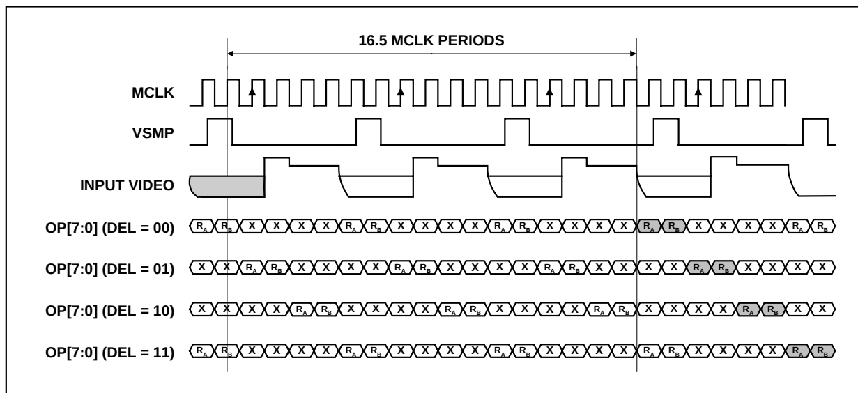
Figure 18 Mode 2 Operation
