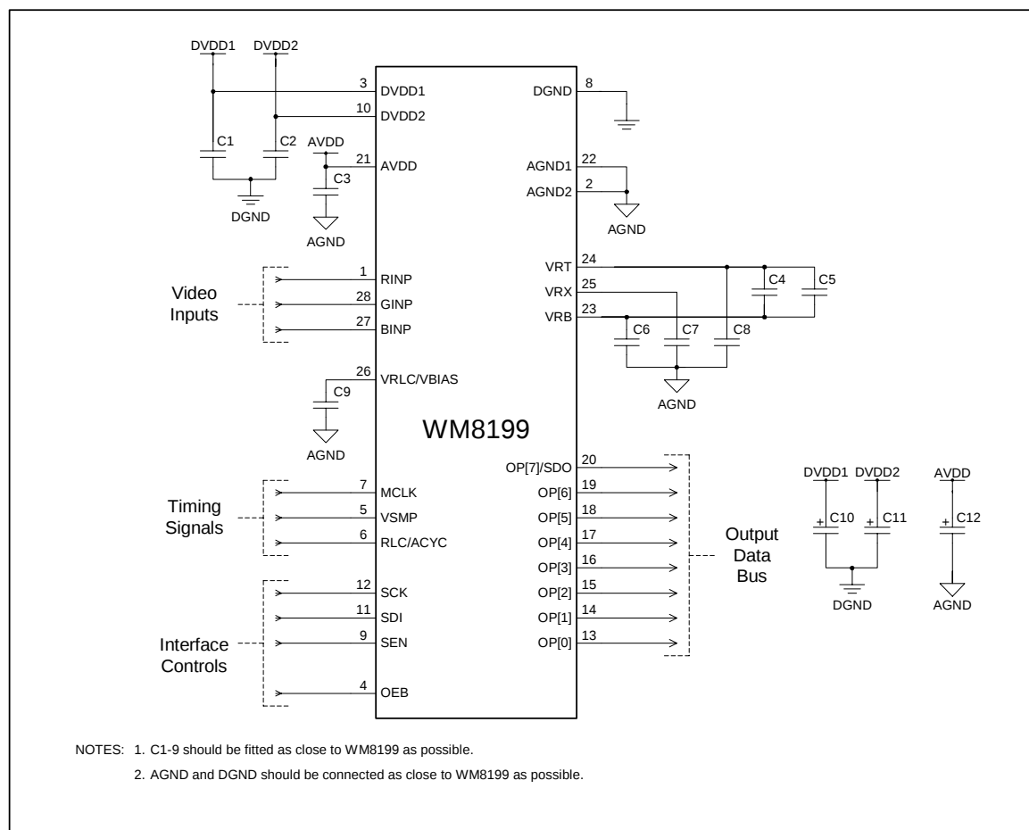
Figure 23 External Components Diagram
