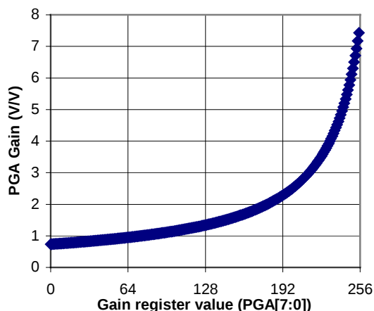
Figure 8 PGA Gain Characteristic
