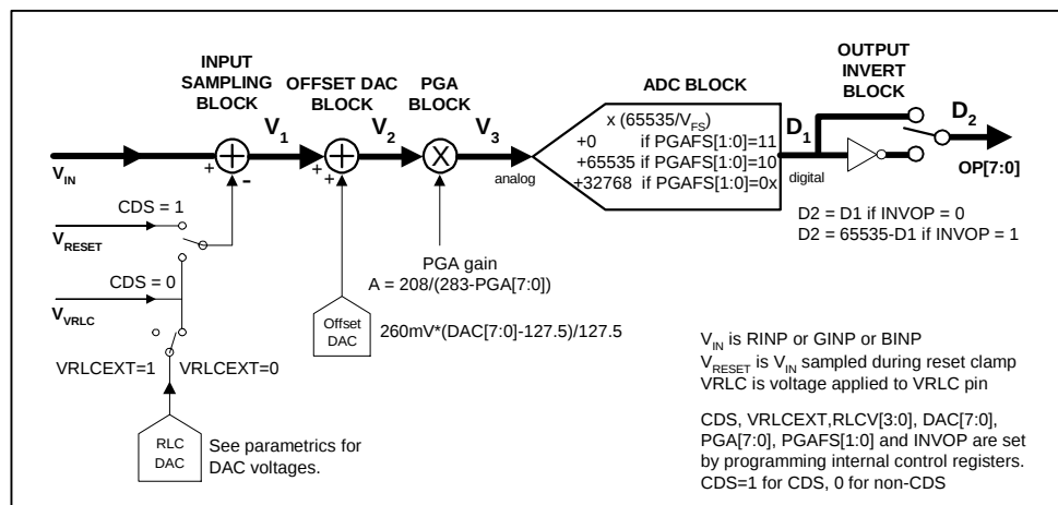
Figure 10 Overall Signal Flow
