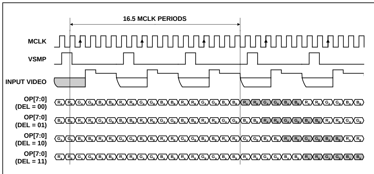
Figure 17 Mode 1 Operation
