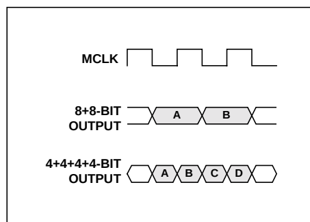
Figure 11 Output Data Formats (Modes 1 – 2, 4 – 6)
