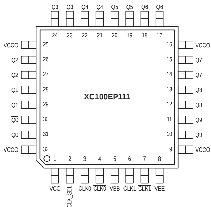
Figure 1. 32-Lead LQFP Pinout (Top View)
