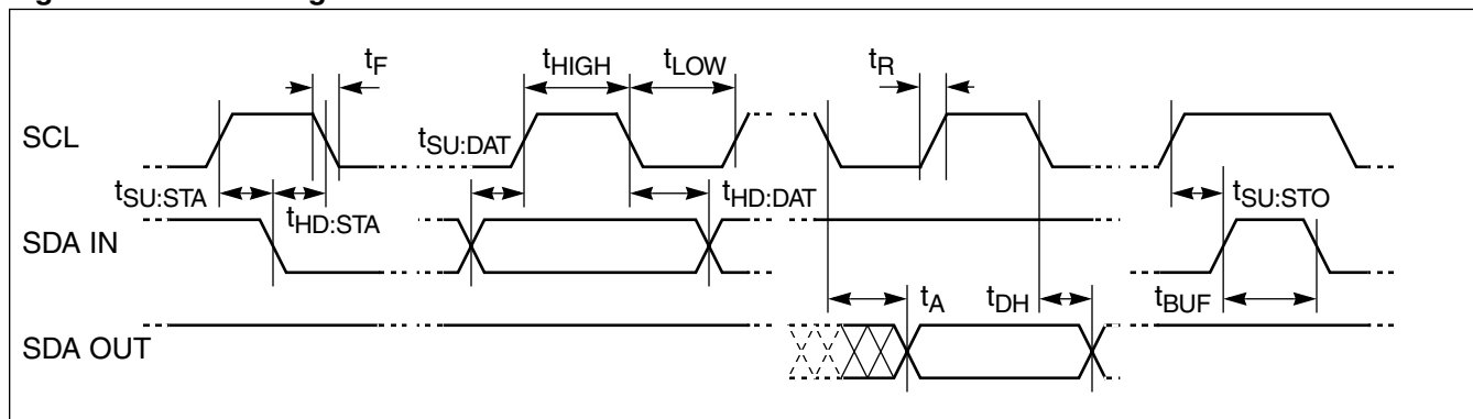
Figure 20. Bus Timing
