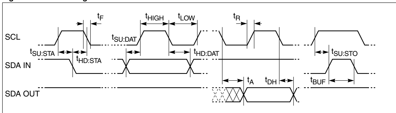
Figure 27. Bus Timing
