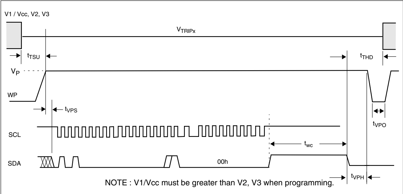
Figure 33. V_{TRIPx} Programming Timing Diagram (x=1,2,3).
