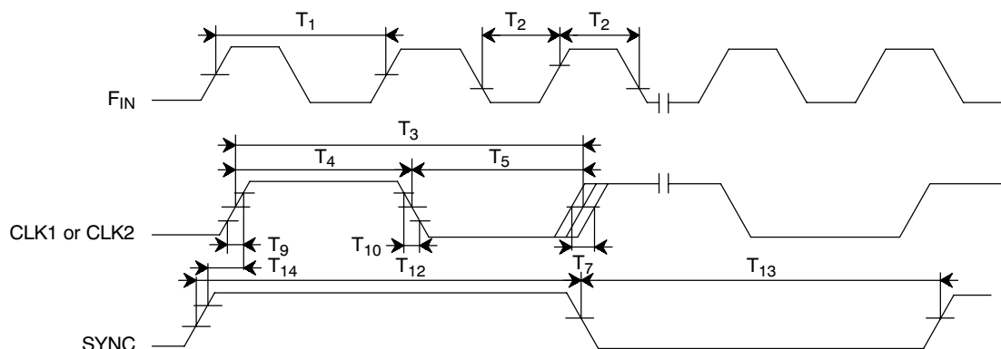
Figure 3. Clocks Timing
