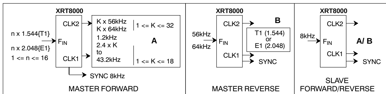
Figure 1. System Diagram
