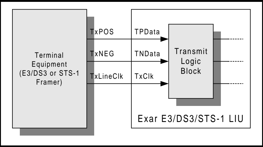
FIGURE 7. THE TYPICAL INTERFACE FOR DATA TRANSMISSION IN DUAL-RAIL FORMAT FROM THE TRANSMITTING TERMINAL EQUIPMENT TO THE TRANSMIT SECTION OF A CHANNEL OF THE XRT73L02
