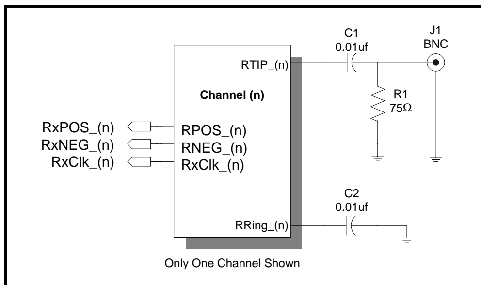
FIGURE 16. RECOMMENDED SCHEMATIC FOR CAPACITIVE-COUPLING THE RECEIVE SECTION OF THE XRT73L02 TO THE LINE
