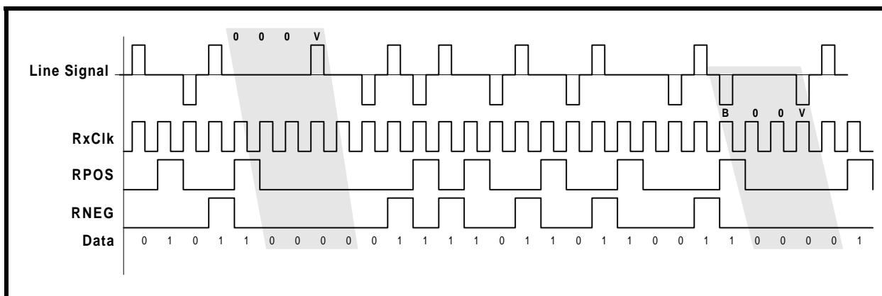
FIGURE 19. AN EXAMPLE OF HDB3 DECODING
