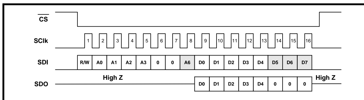
FIGURE 31. MICROPROCESSOR SERIAL INTERFACE DATA STRUCTURE
