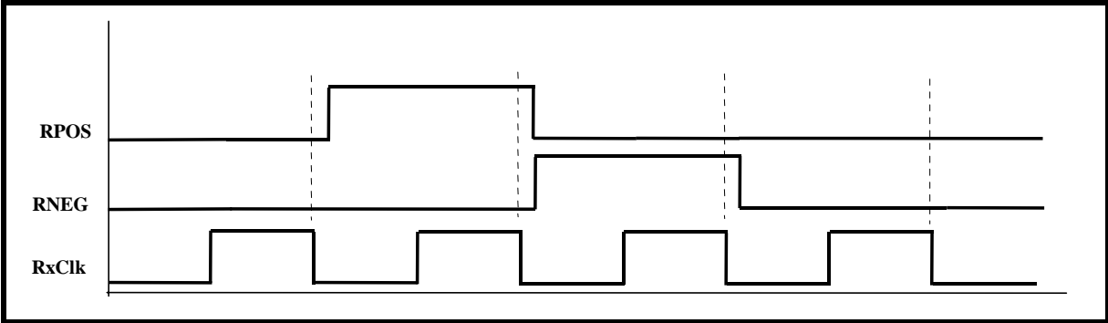
FIGURE 24. THE BEHAVIOR OF THE RPOS, RNEG AND RXCLK SIGNALS WHEN RXCLK IS INVERTED
