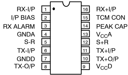
16 Lead PDIP (0.300\
