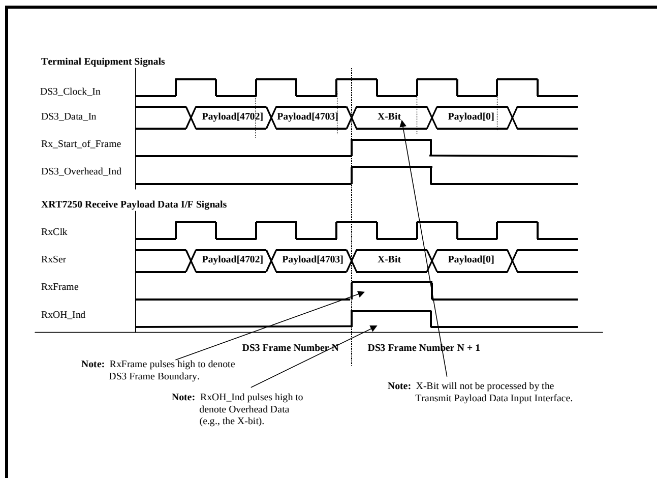
FIGURE 94. AN ILLUSTRATION OF THE BEHAVIOR OF THE SIGNALS BETWEEN THE RECEIVE PAYLOAD DATA OUTPUT INTERFACE BLOCK OF THE XRT7250 AND THE TERMINAL EQUIPMENT (SERIAL MODE OPERATION)
