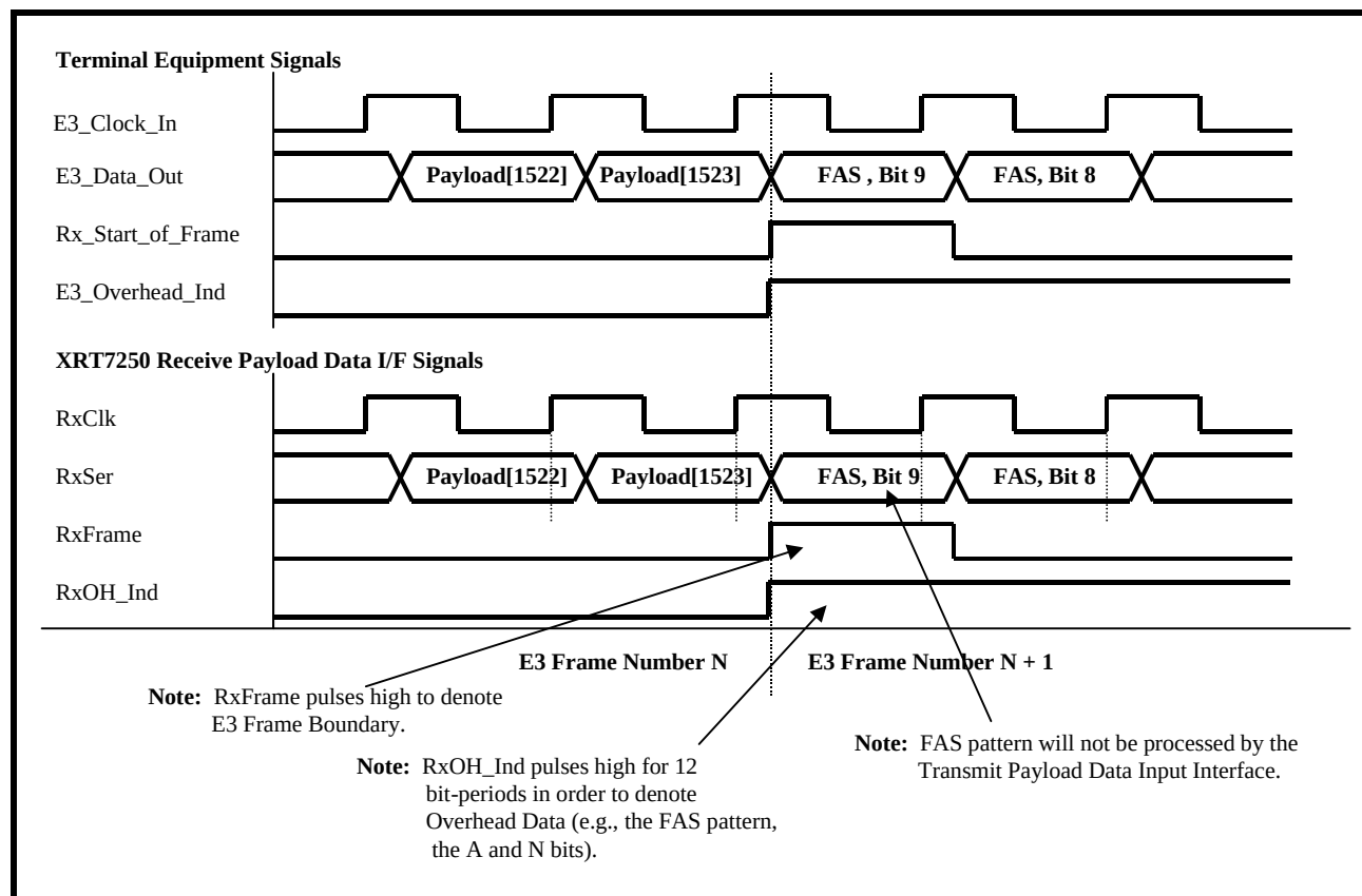
FIGURE 151. AN ILLUSTRATION OF THE BEHAVIOR OF THE SIGNALS BETWEEN THE RECEIVE PAYLOAD DATA OUTPUT INTERFACE BLOCK OF THE XRT7250 AND THE TERMINAL EQUIPMENT
