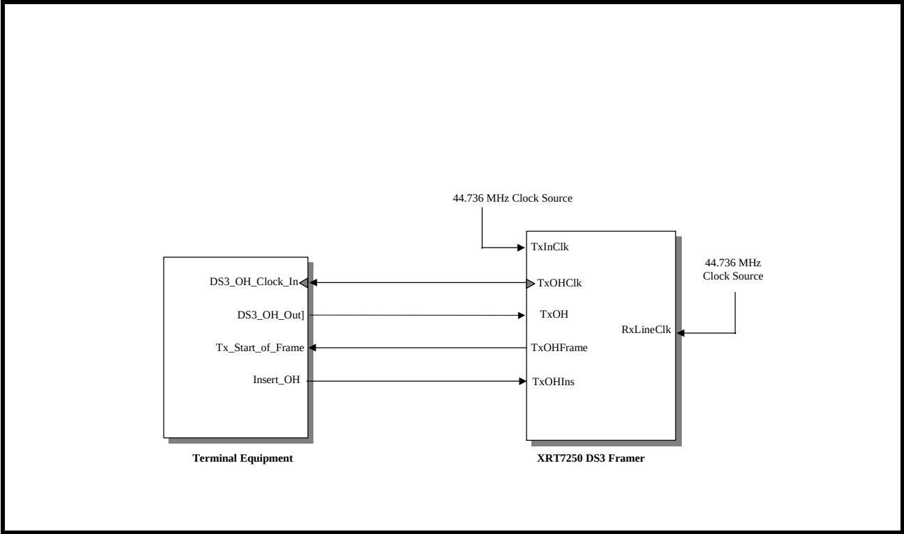
FIGURE 57. ILLUSTRATION OF THE TERMINAL EQUIPMENT BEING INTERFACED TO THE TRANSMIT OVERHEAD DATA INPUT INTERFACE (METHOD 1)
