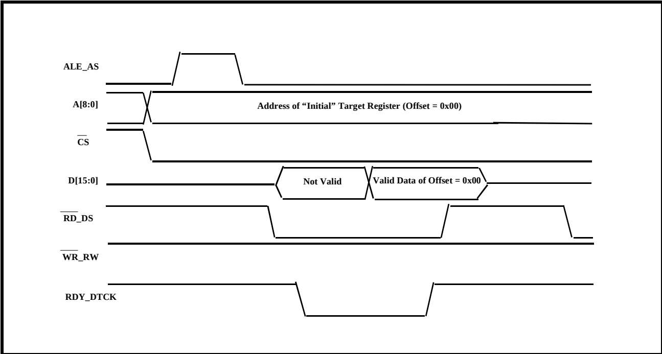
FIGURE 29. BEHAVIOR OF THE MICROPROCESSOR INTERFACE SIGNALS, DURING THE INITIAL READ OPERATION OF A BURST CYCLE (INTEL TYPE PROCESSOR)
