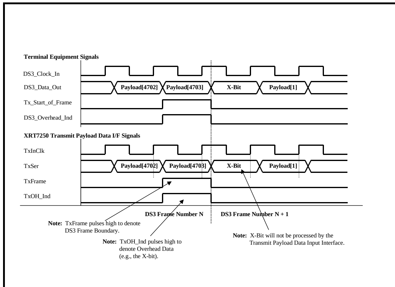
FIGURE 49. BEHAVIOR OF THE TERMINAL INTERFACE SIGNALS BETWEEN THE XRT7250 AND THE TERMINAL EQUIPMENT (DS3 MODE 3 OPERATION)
