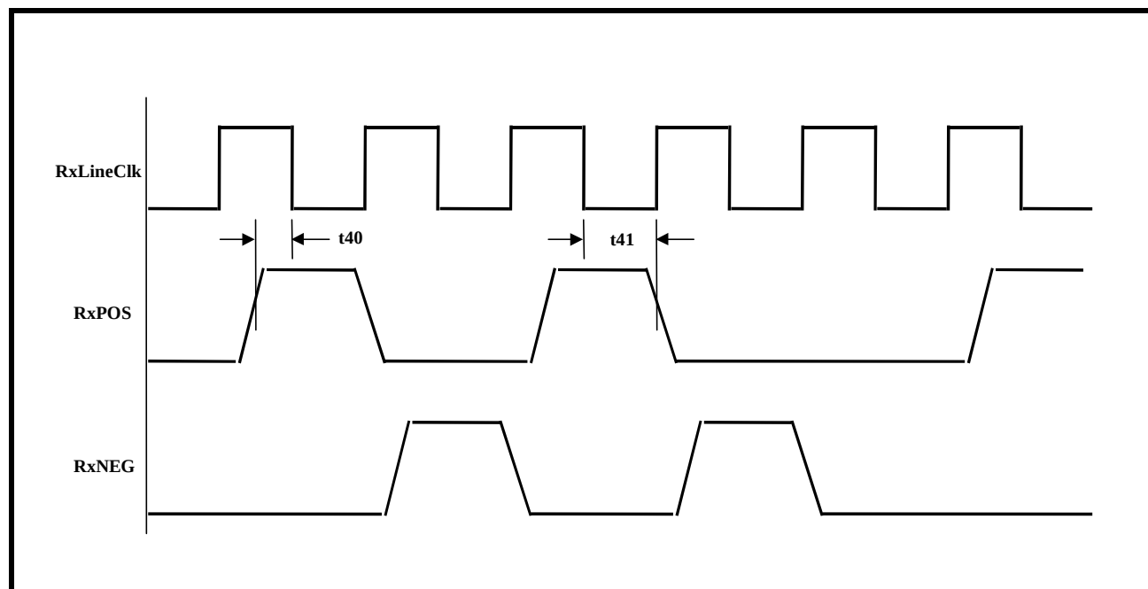
FIGURE 9. RECEIVE LIU INTERFACE TIMING - FRAMER IS CONFIGURED TO SAMPLE "RxPOS" AND "RxNEG" ON THE RISING EDGE OF "RxLINECLK"
