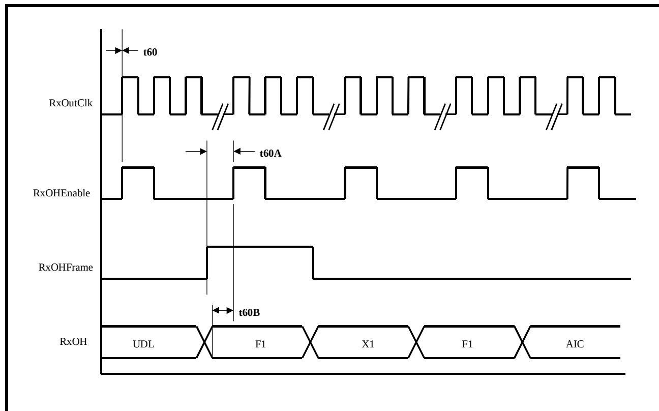
FIGURE 14. RECEIVE OVERHEAD DATA OUTPUT INTERFACE TIMING (METHOD 2 - USING RxOHENABLE)
