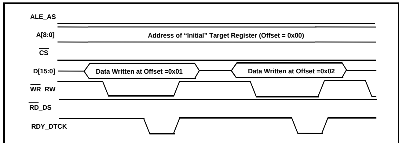
FIGURE 32. BEHAVIOR OF THE MICROPROCESSOR INTERFACE SIGNALS, DURING SUBSEQUENT WRITE OPERATIONS WITHIN THE BURST I/O CYCLE
