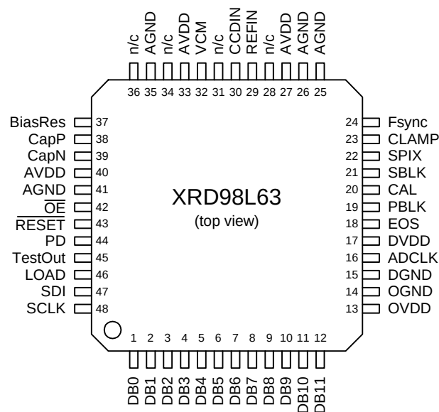
Figure 2. XRD98L63 Pinout
