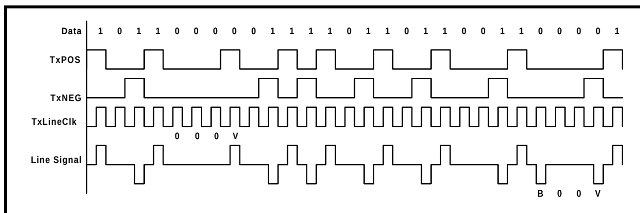
FIGURE 182. ILLUSTRATION OF TWO EXAMPLES OF HDB3 ENCODING
