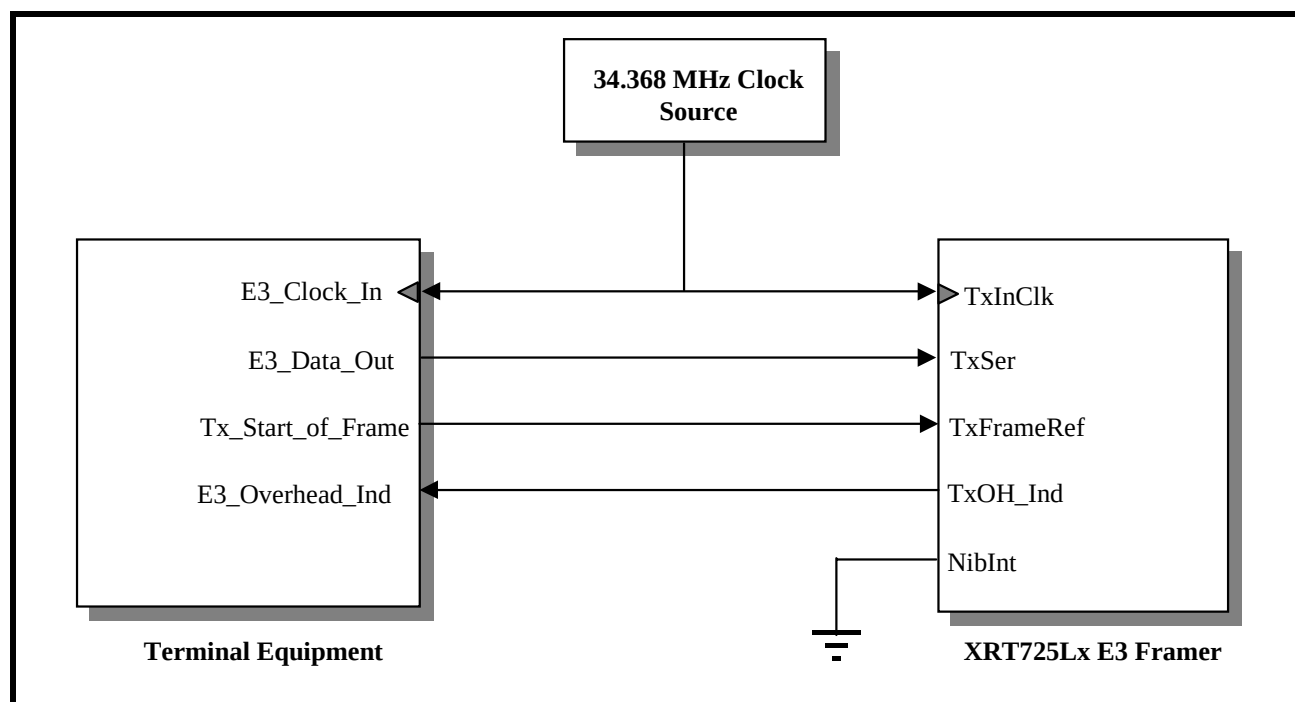
FIGURE 102. ILLUSTRATION OF THE TERMINAL EQUIPMENT BEING INTERFACED TO THE TRANSMIT PAYLOAD DATA INPUT INTERFACE BLOCK OF THE XRT72L53 FOR MODE 2 (SERIAL/LOCAL-TIMED/FRAME-SLAVE) OPERATION
