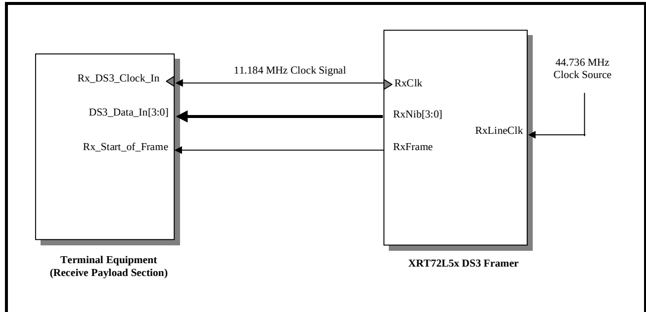
FIGURE 95. ILLUSTRATION OF THE XRT72L52 DS3/E3 FRAMER IC BEING INTERFACED TO THE RECEIVE SECTION OF THE TERMINAL EQUIPMENT (NIBBLE-MODE OPERATION)
