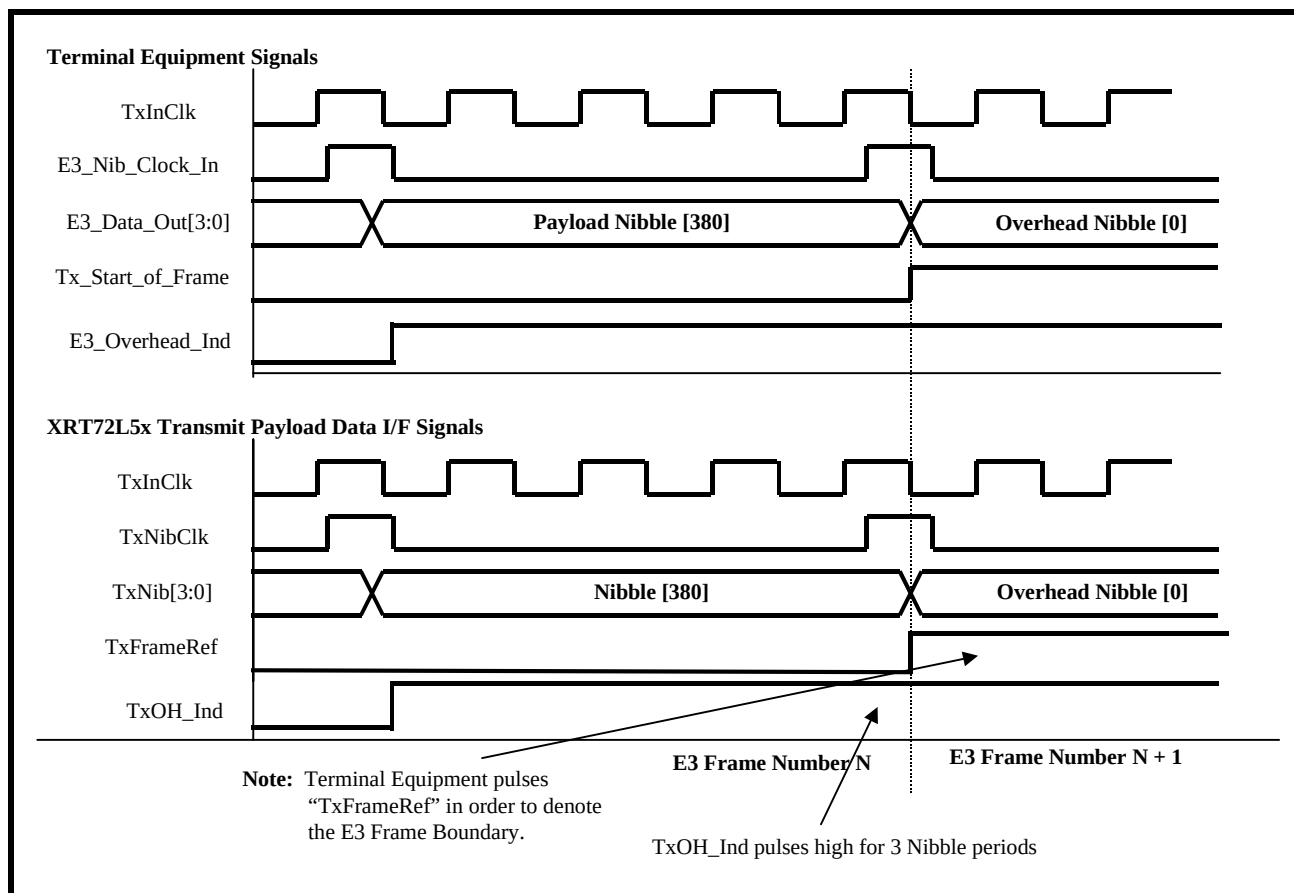
FIGURE 109. BEHAVIOR OF THE TERMINAL INTERFACE SIGNALS BETWEEN THE XRT72L52 AND THE TERMINAL EQUIPMENT (E3, MODE 5 OPERATION)
