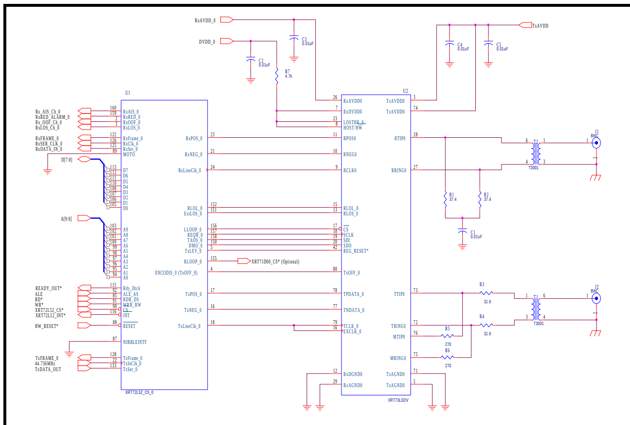
FIGURE 65. APPROACH TO INTERFACING THE XRT72L52 FRAMER IC TO THE XRT73L02 DS3/E3/STS-1 TRANSMITTER LIU (ONE CHANNEL SHOWN)
