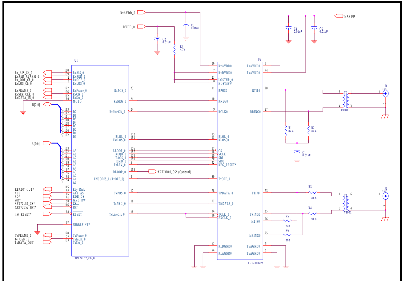
FIGURE 120. APPROACH TO INTERFACING THE XRT72L52 FRAMER IC TO THE XRT73L02 DS3/E3/STS-1 LIU
