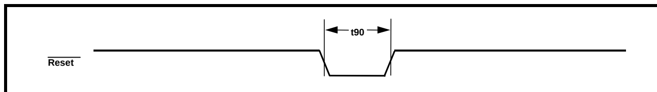
FIGURE 23. MICROPROCESSOR INTERFACE TIMING - RESET PULSE WIDTH
