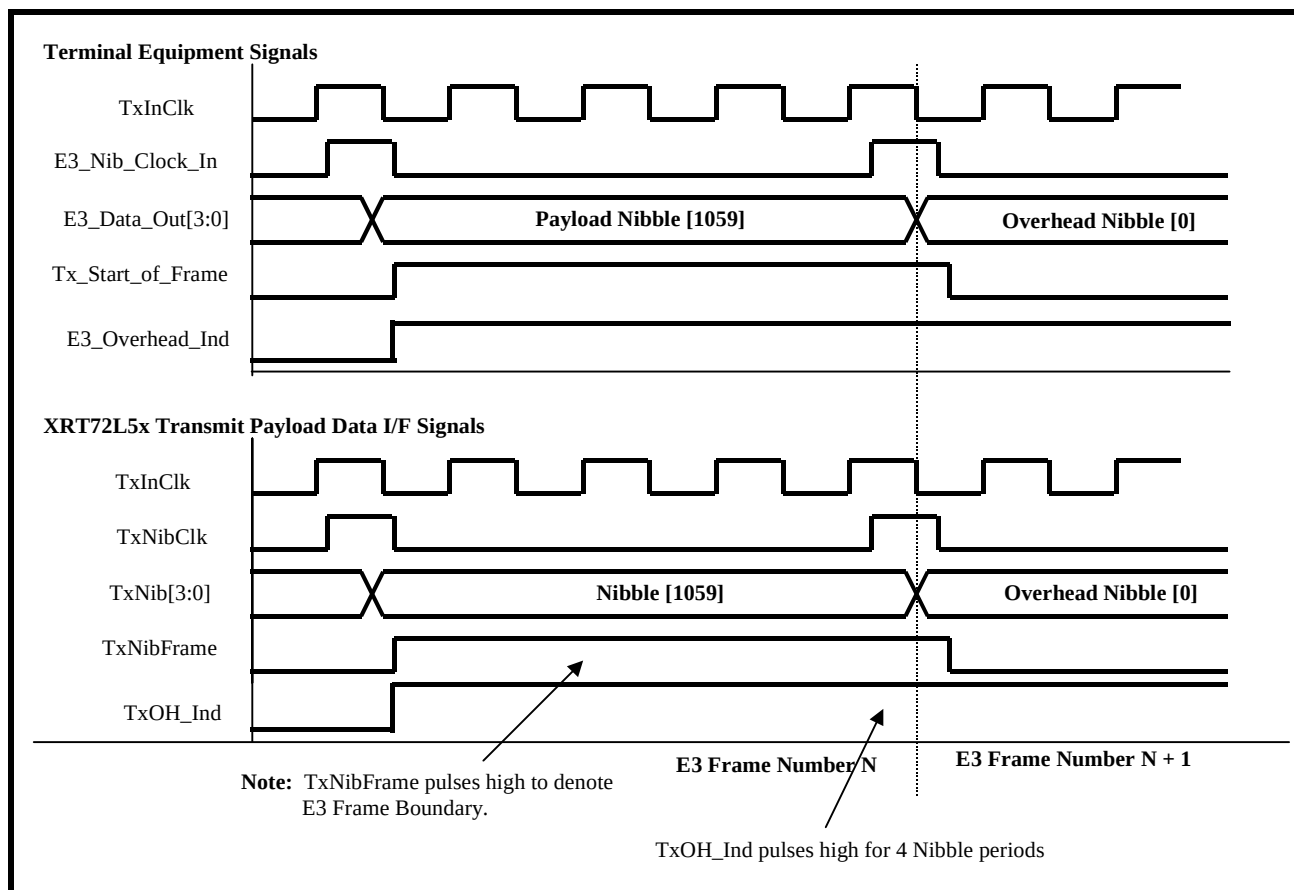
FIGURE 168. BEHAVIOR OF THE TERMINAL INTERFACE SIGNALS BETWEEN THE XRT72L52 AND THE TERMINAL EQUIPMENT (E3 MODE 6 OPERATION)
