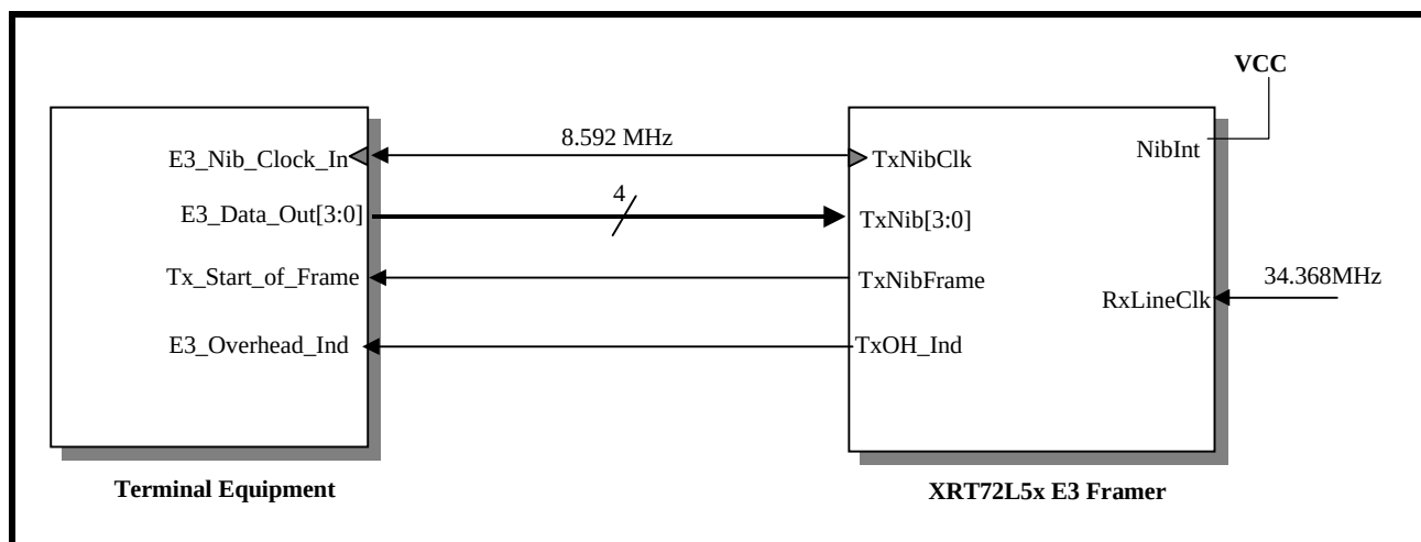
FIGURE 106. ILLUSTRATION OF THE TERMINAL EQUIPMENT BEING INTERFACED TO THE TRANSMIT PAYLOAD DATA INPUT INTERFACE BLOCK OF THE XRT72L52 FOR MODE 4 (NIBBLE-PARALLEL/LOOP-TIMED) OPERATION
