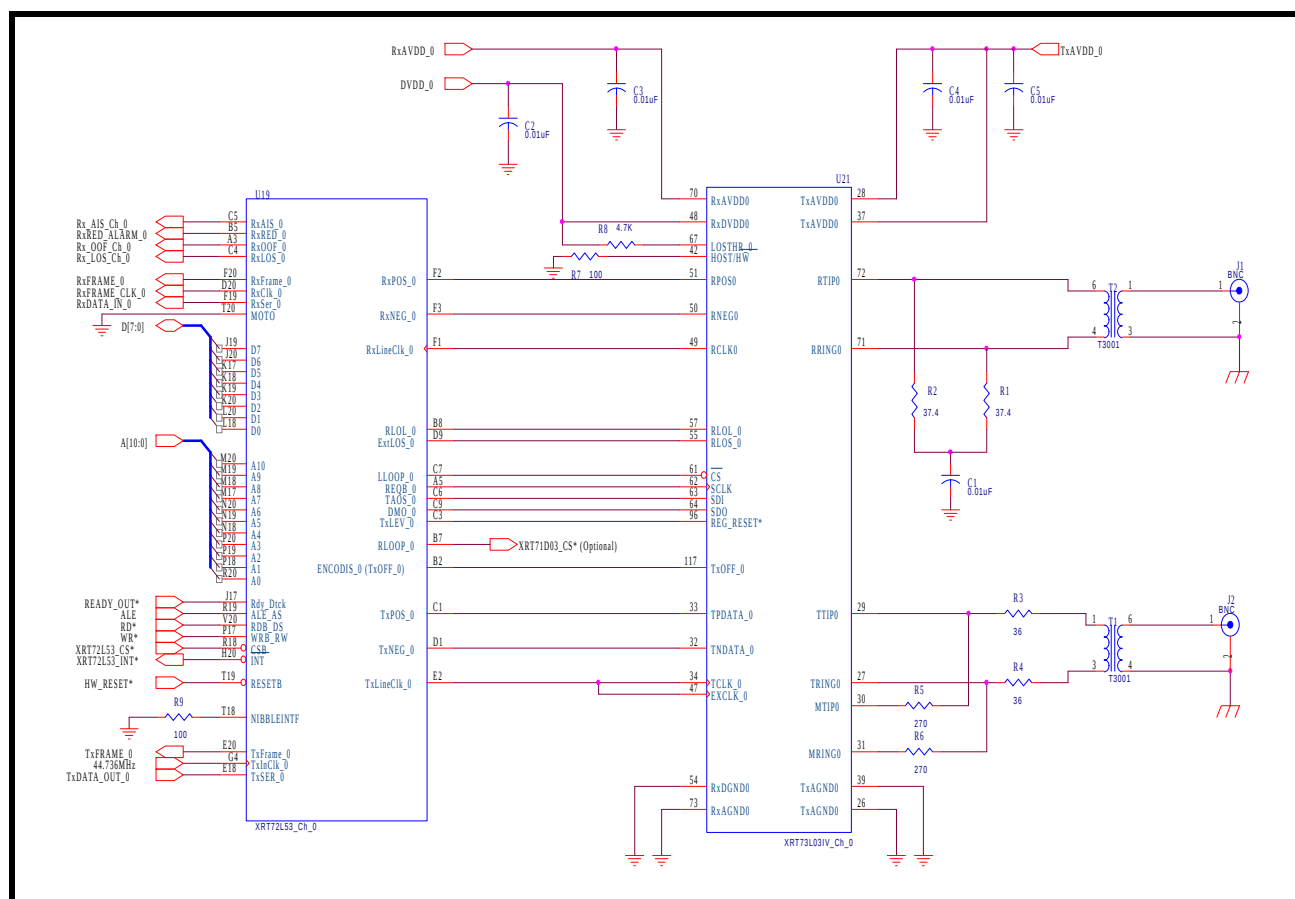
FIGURE 178. APPROACH TO INTERFACING THE XRT72L52 FRAMER IC DEVICE TO THE XRT73L03 DS3/E3/STS-1 LIU
