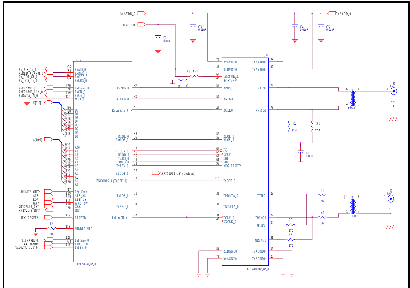
FIGURE 130. ILLUSTRATION ON HOW A CHANNEL OF THE RECEIVE E3 FRAMER (WITHIN THE XRT72L52 FRAMER IC) BEING INTERFACE TO THE XRT73L03 LINE INTERFACE UNIT, WHILE OPERATING IN BIPOLAR MODE
