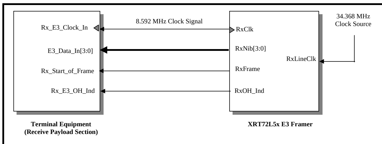
FIGURE 211. ILLUSTRATION OF THE XRT72L52 DS3/E3 FRAMER IC BEING INTERFACED TO THE RECEIVE SECTION OF THE TERMINAL EQUIPMENT (NIBBLE-MODE OPERATION)
