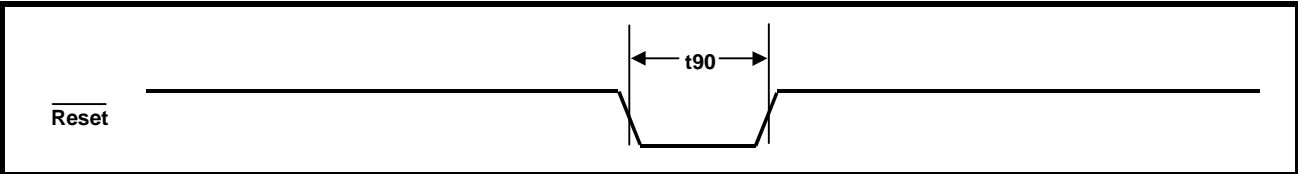
FIGURE 20. MICROPROCESSOR INTERFACE TIMING - RESET PULSE WIDTH
