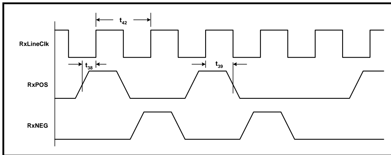
FIGURE 11. RECEIVE DS3 FRAMER LINE INTERFACE INPUT SIGNAL TIMING (RxPOS AND RxNEG ARE SAMPLED ON RISING EDGE OF RxLineClk)
