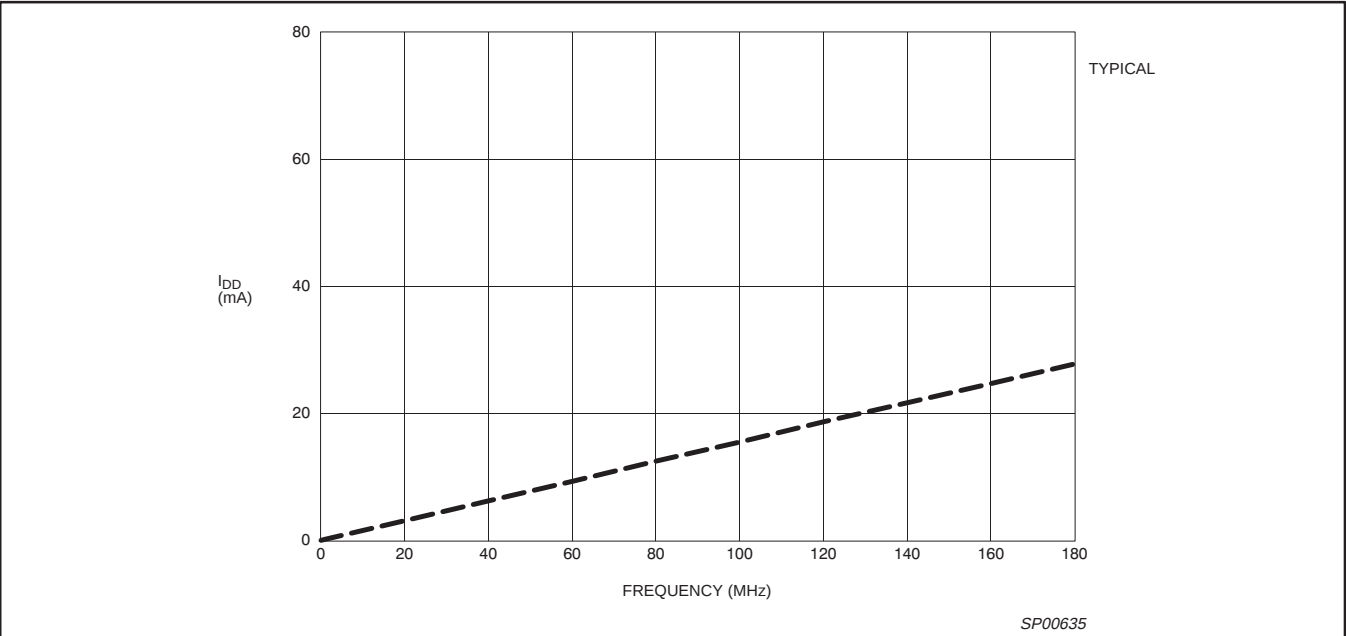
Figure 5. I_{DD} vs. Frequency @ V_{DD} = 5.0\text{V}
