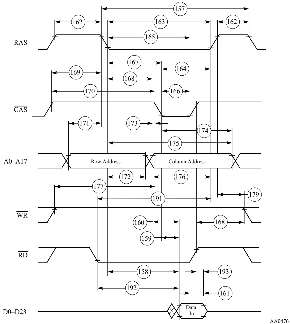
Figure 2-15 DRAM Out-of-Page Read Access
