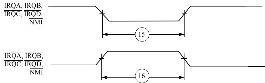
Figure 2-4 External Interrupt Timing (Negative Edge-Triggered)
