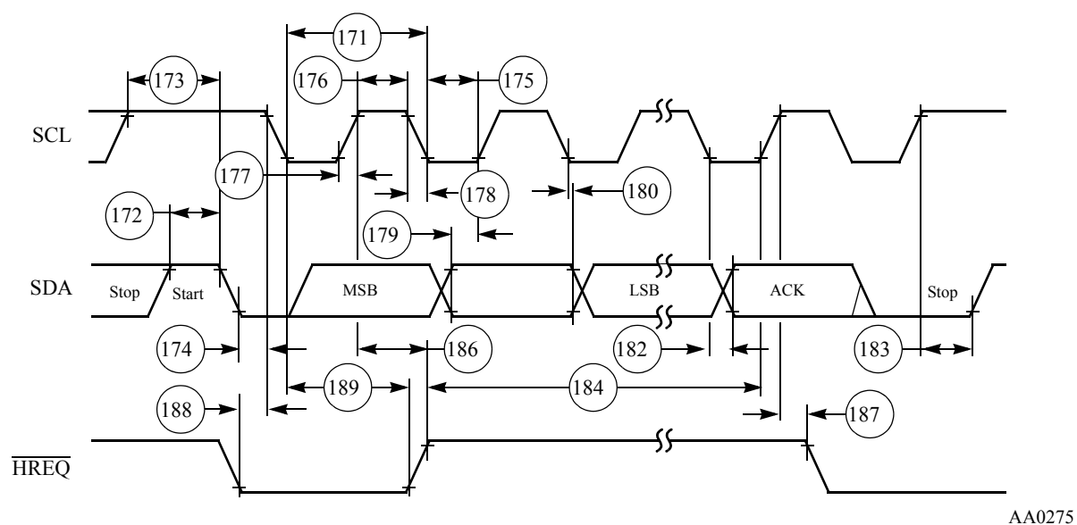
Figure 2-31 I 2 C Timing
