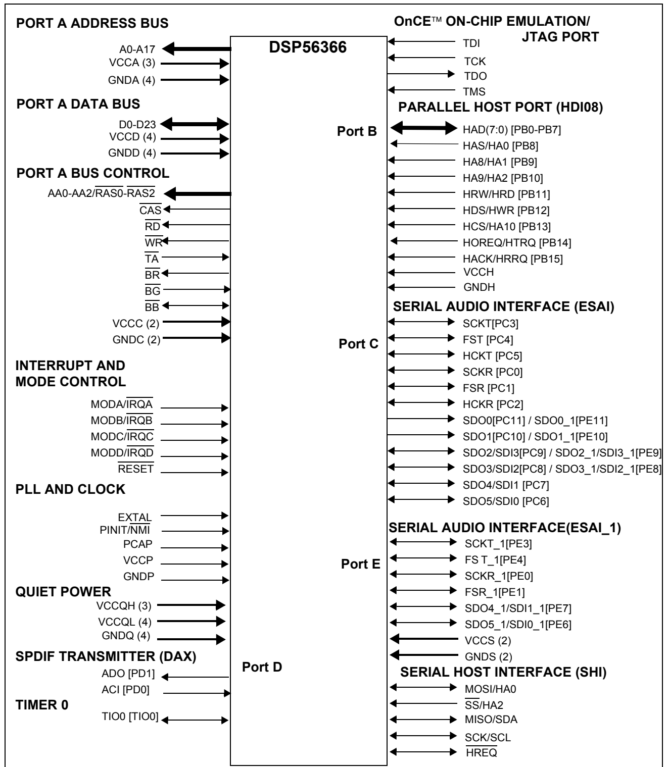
Figure 1-1 Signals Identified by Functional Group
