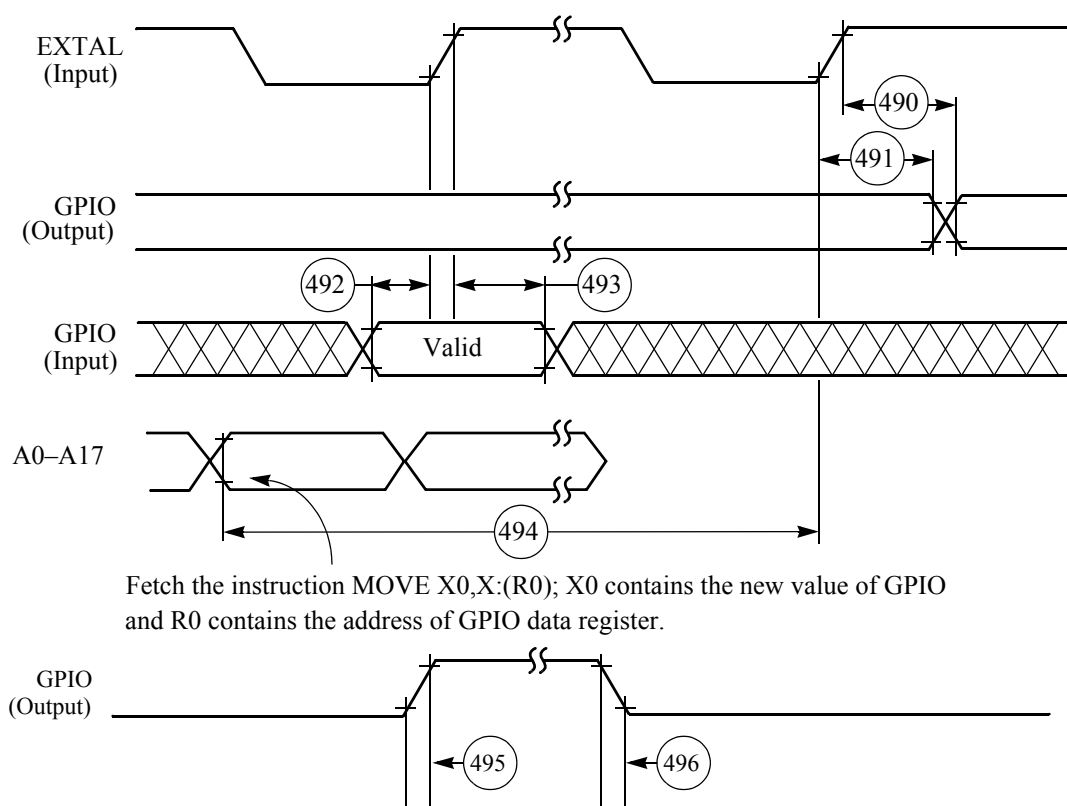
Figure 2-38 GPIO Timing
