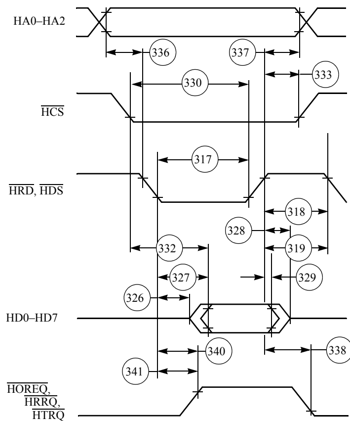
Figure 2-21 Read Timing Diagram, Non-Multiplexed Bus
