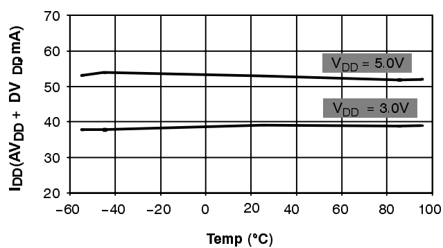
Figure 19. I_{DD} vs Temperature, F_S=16\text{MSPS} , V_{RT}=V_{DD}/1.3 , V_{RB}=V_{DD}/10
