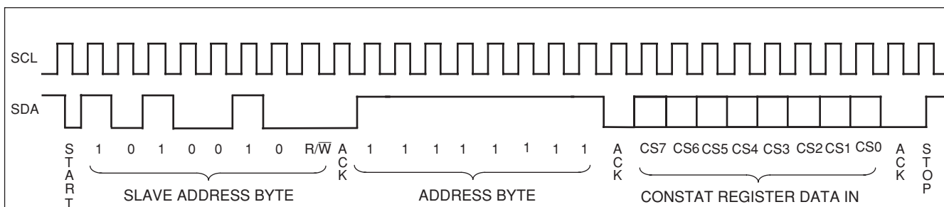
Figure 18. CONSTAT Register Write Command Sequence
