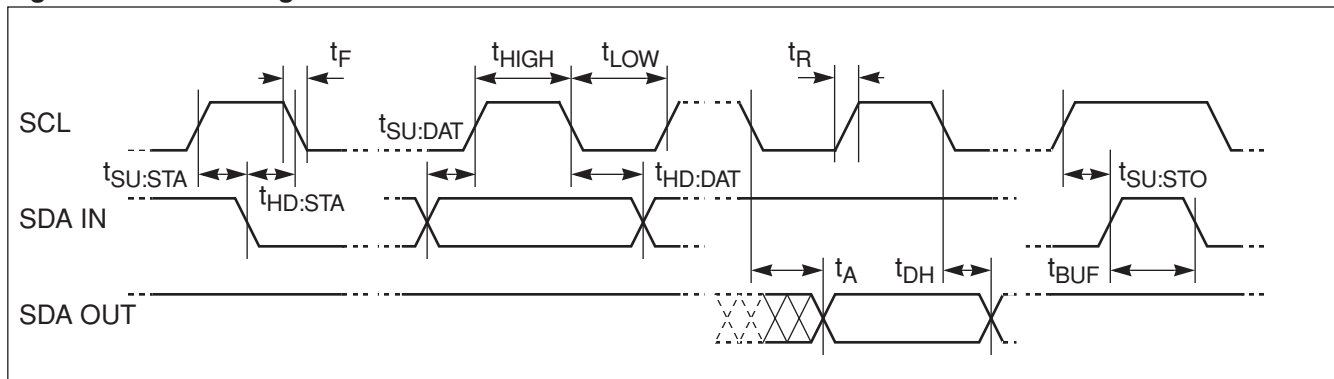
Figure 22. Bus Timing
