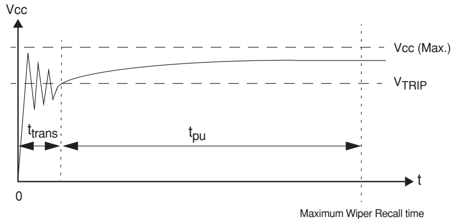
Figure 7. DCP Power up
