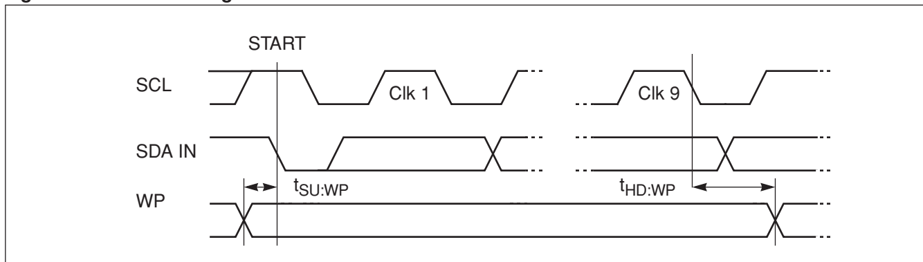
Figure 23. WP Pin Timing
